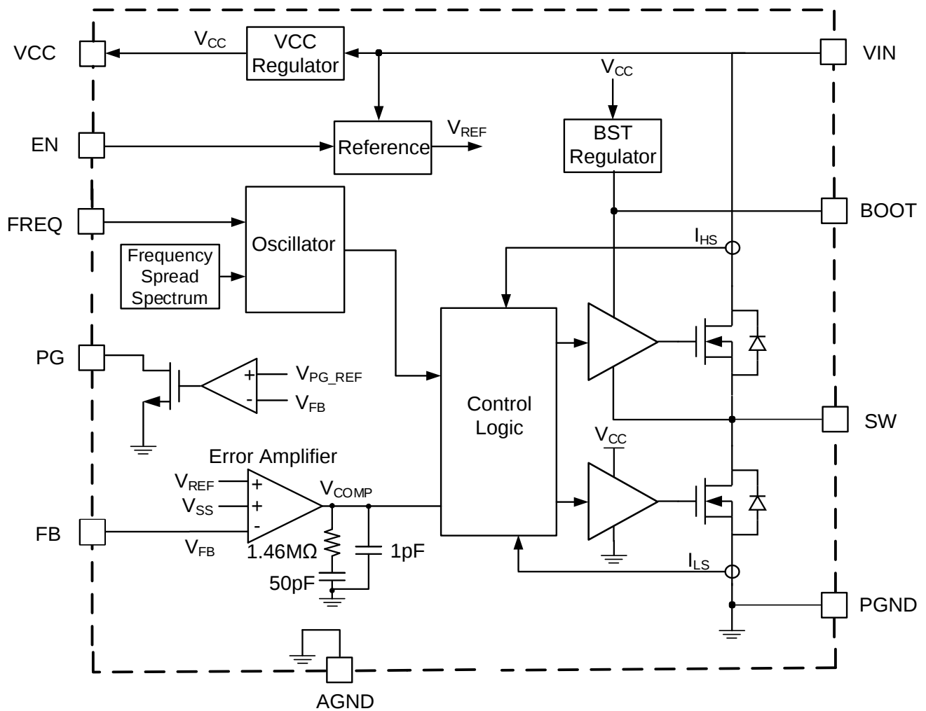
Figure 3: Functional Block Diagram (Adjustable Output)
