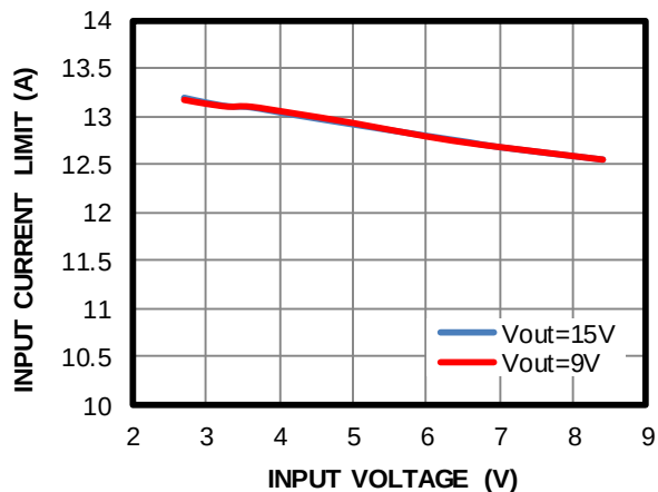
Input Current Limit vs. Input Voltage R_{ILIM} = 22k\Omega
