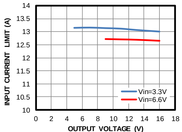
Input Current Limit vs. Output Voltage R_{ILIM} = 22k\Omega
