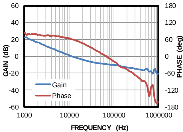
Bode Plot
