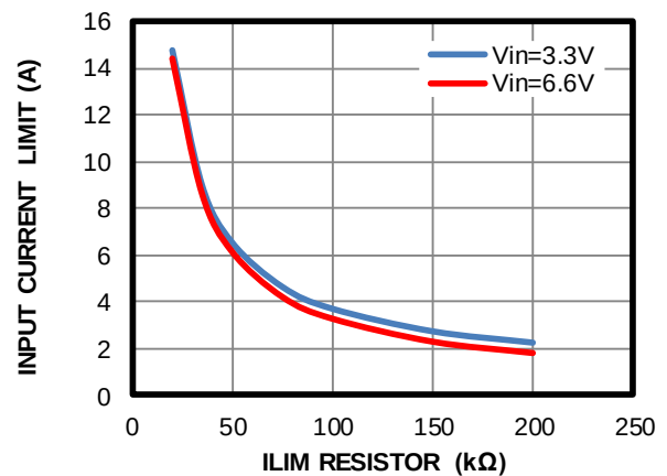
Input Current Limit vs. ILIM Resistor V_{OUT} = 9V
