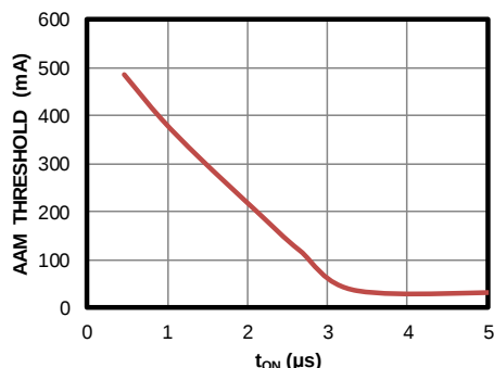
Figure 9: AAM Threshold Decreases as t_{ON} Increases
