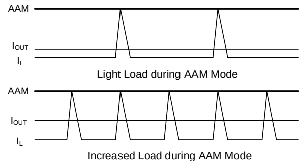
Figure 6: AAM Comparator Controls SW's t_{ON}
