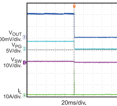
Short-Circuit Protection Entry, Latch Off Mode
