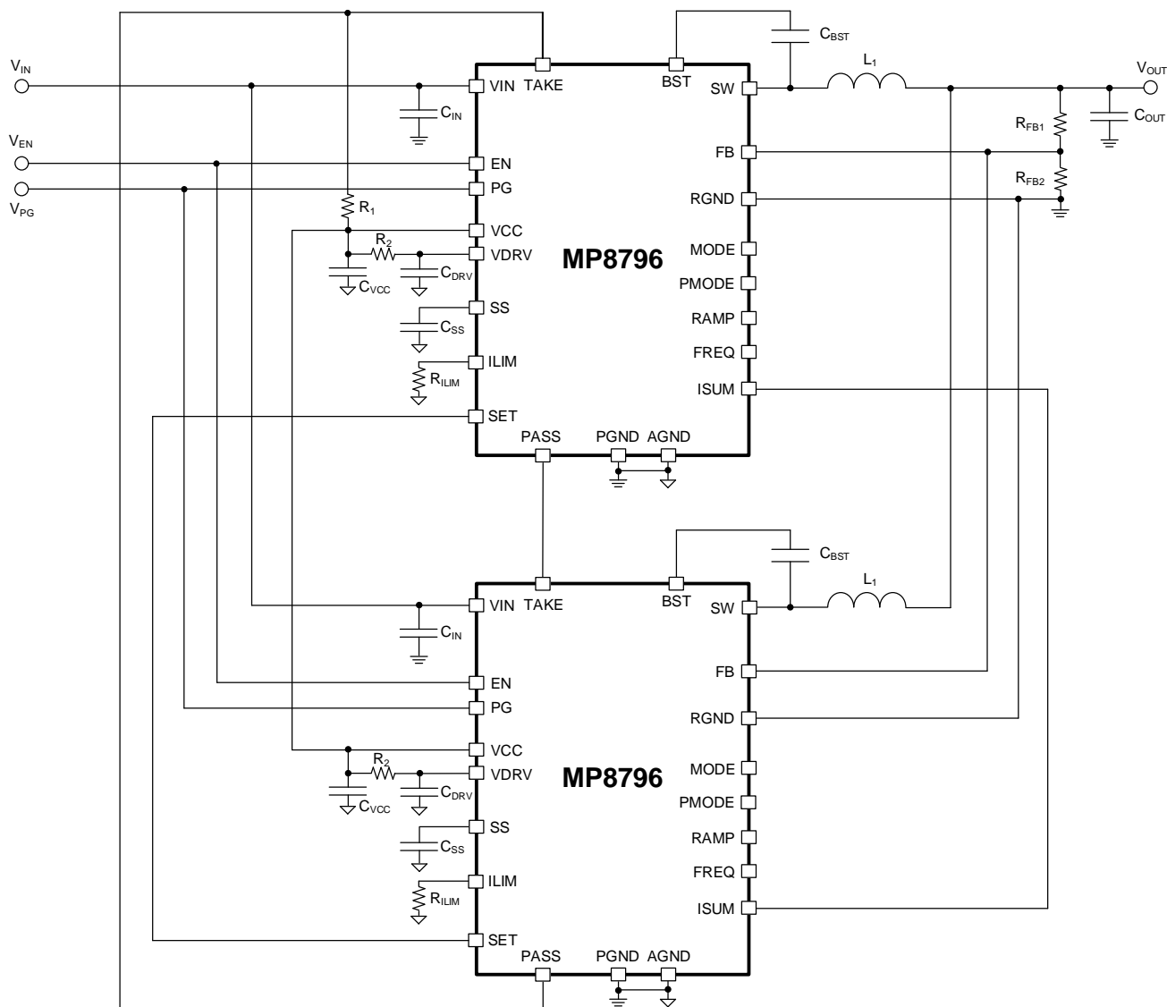
Figure 2: Dual-Phase Operation
