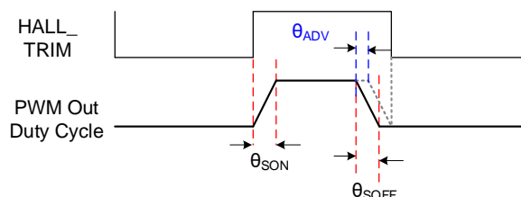
Figure 6: Advanced Soft Off Angle
