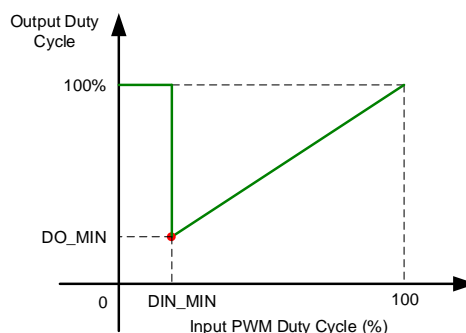
Figure 3: Speed Curve (SPD_ZERO = 0, MAX_EN = 1)
