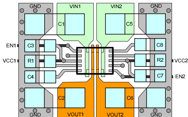
Figure 4: Recommended Layout
