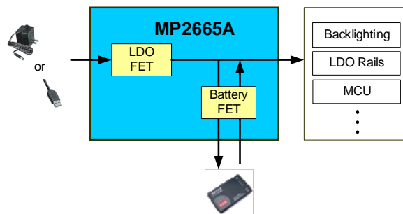
Figure 3: Power Path Management Structure
