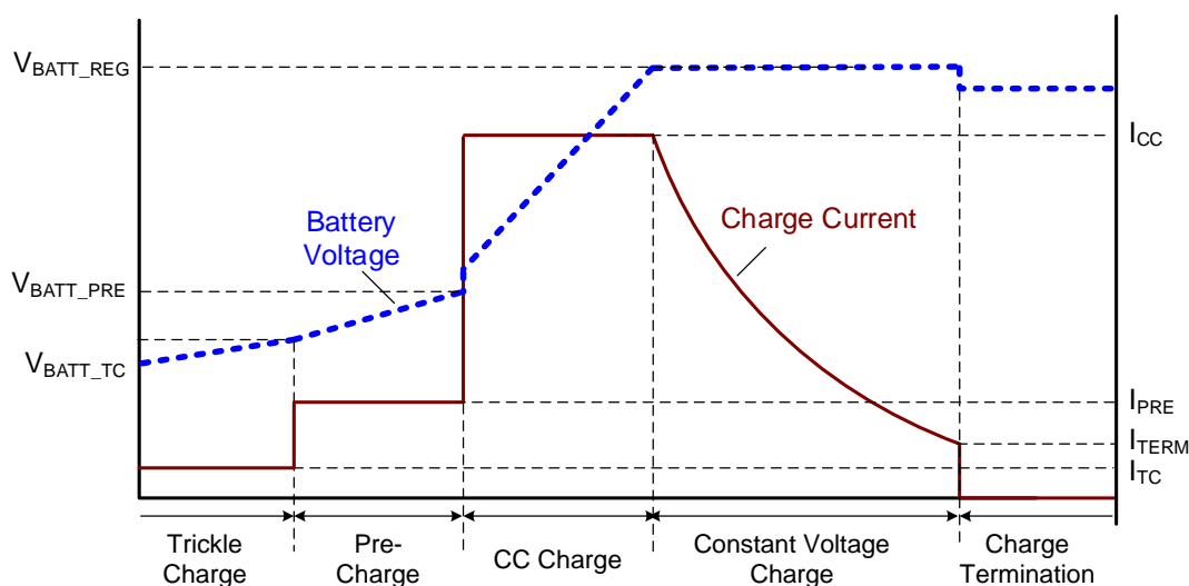
Figure 5: Charge Profile
