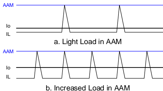
Figure 3: AAM Comparator Control t_{ON}
