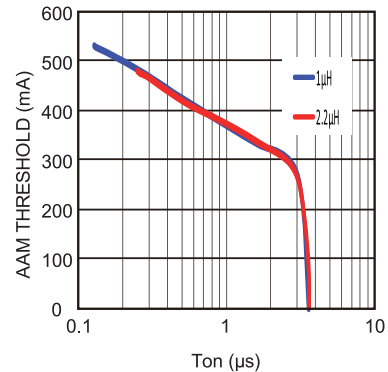
Figure 9: AAM Threshold decreases with Ton Increases.
