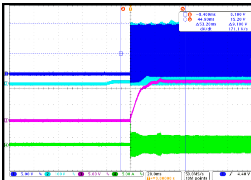
Start-Up Full load
