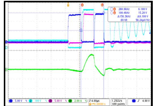
Steady State No load
