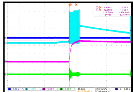
Start-Up No load
