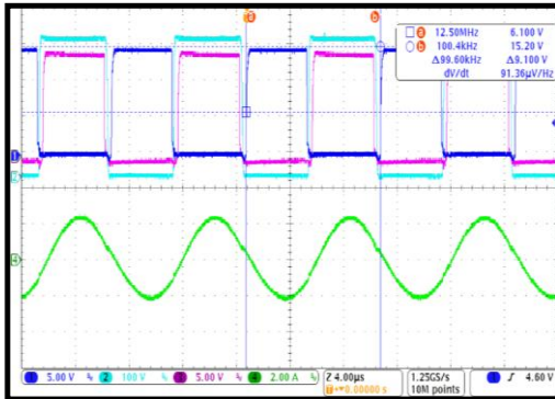
Steady State Full load
