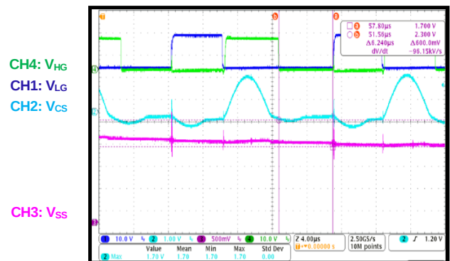
Capacitive Mode Protection Short circuit
