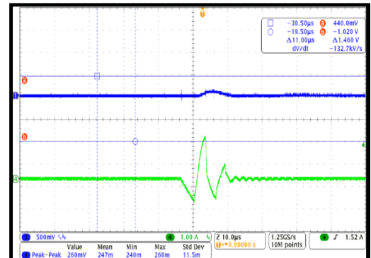
Output Ripple No load
