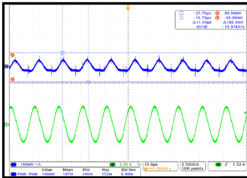
Output Ripple Full load
