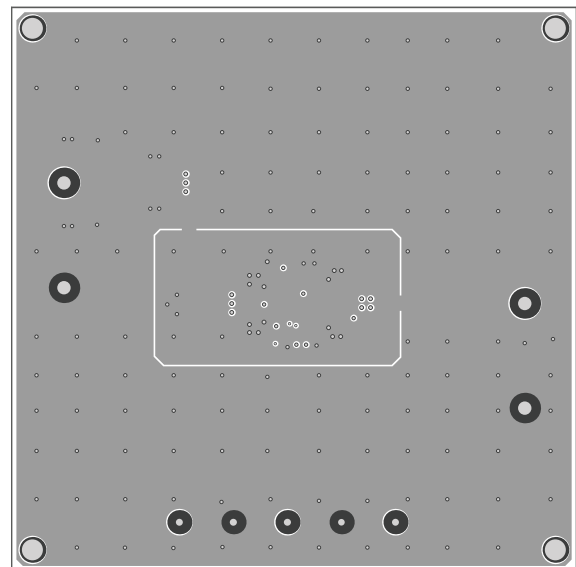
Figure 2: Inner 1 Layer
