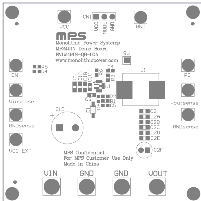
Figure 3: Top Silk
