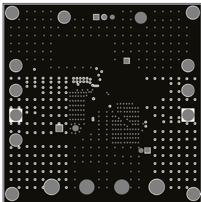
Figure 5: Mid-Layer 1
