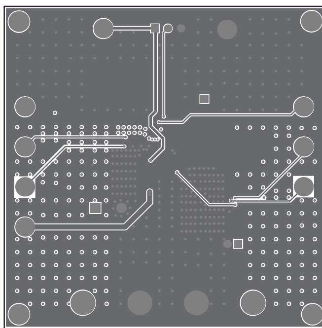
Figure 6: Mid-Layer 2
