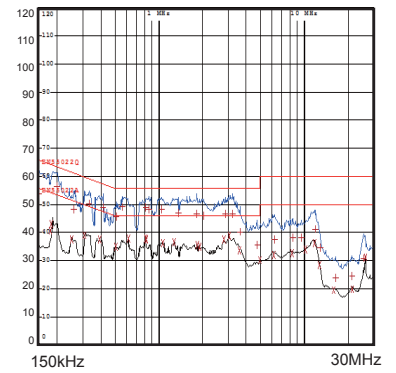
Conducted EMI Line wire
