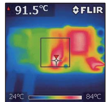
Thermal Performance V_{IN} = 265V_{AC}
