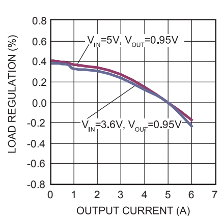
Load Regulation Vs. I OUT
