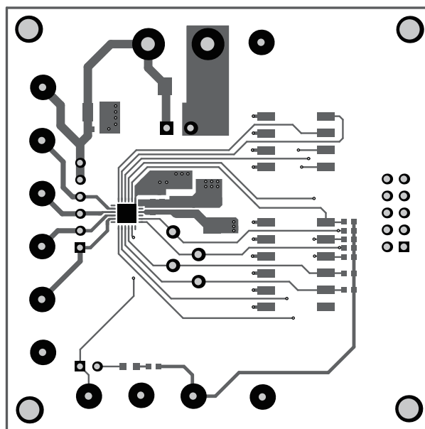
Figure 5: Top Layer
