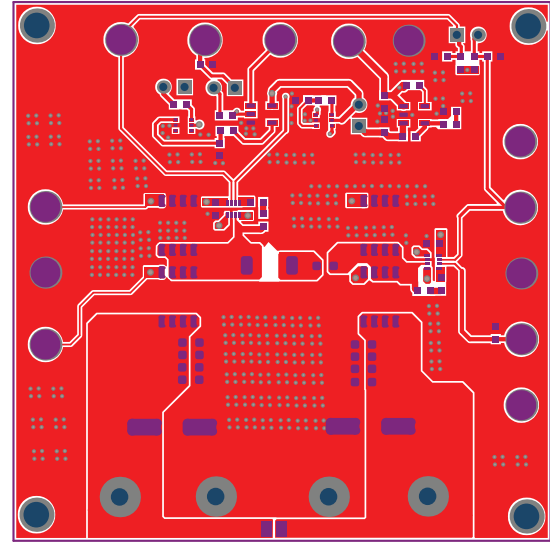
Figure 3: Top Layer
