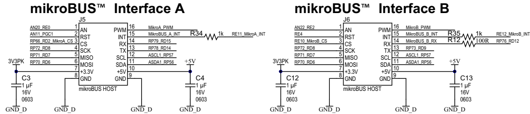
FIGURE A-4: dsPIC33CK CURIOSITY DEVELOPMENT BOARD SCHEMATICS, REV. 2.0 (PAGE 4 OF 8)
