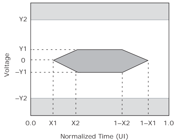
Figure 115 • SFI Transmit Differential Output Compliance Mask
