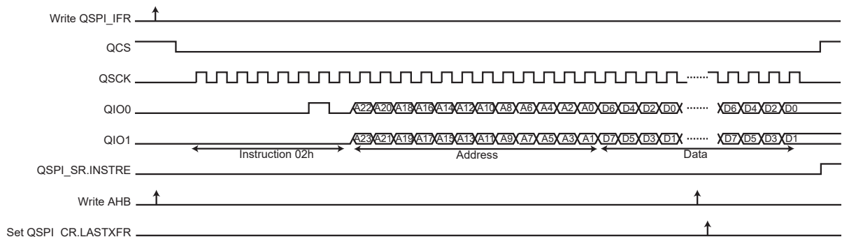
Figure 46-15. Instruction Transmission Waveform 5
