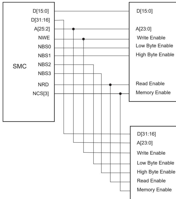
Figure 33-7. Connection of 2x16-bit Data Bus on a 32-bit Data Bus (Byte Select Option)
