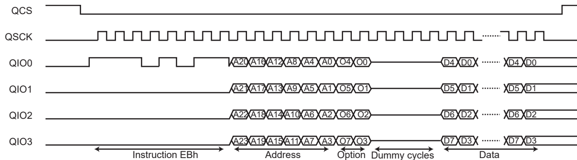
Figure 46-8. Instruction Frame
