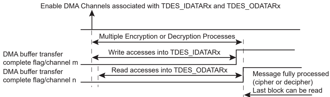
Figure 54-4. DMA Transfer with LOD = 0
