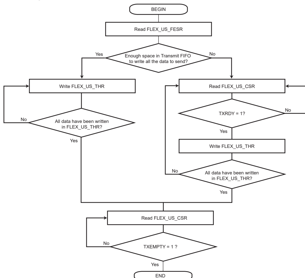
Figure 45-71. Sending Data with FIFO Enabled
