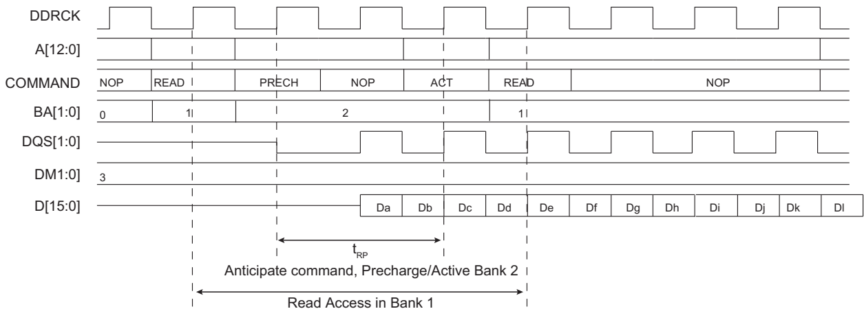
Figure 31-19. Anticipate Precharge/Activate Command in Bank 2 during Read Access in Bank 1
