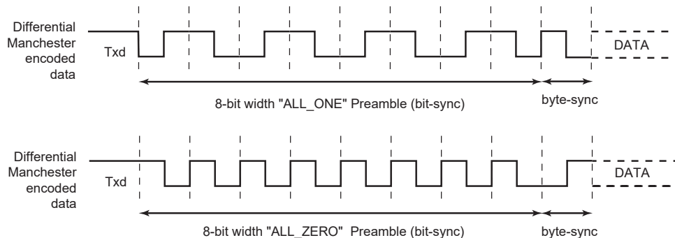
Figure 45-57. Preamble Patterns
