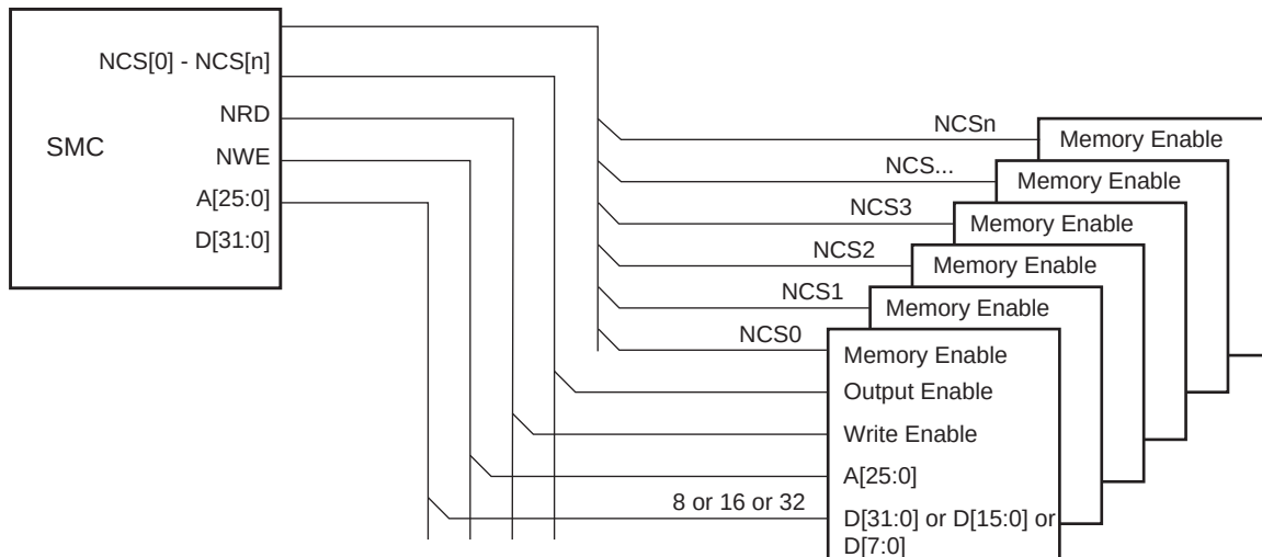
Figure 33-2. Memory Connections for Eight External Devices
