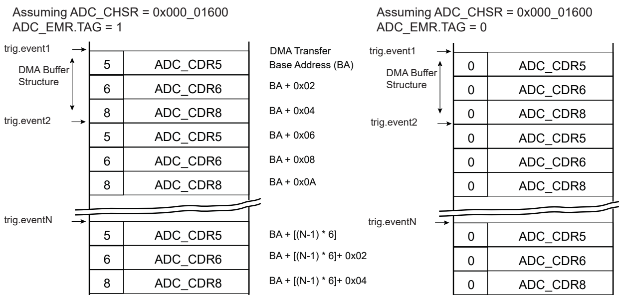
Figure 56-21. Buffer Structure
