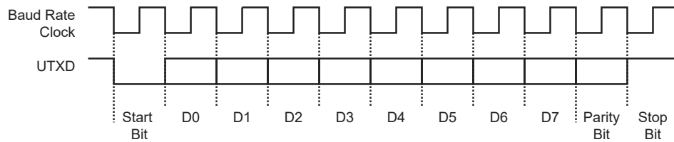
Figure 21-10. Character Transmission
