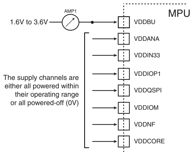
Figure 57-42. Measurement on VDDBU
