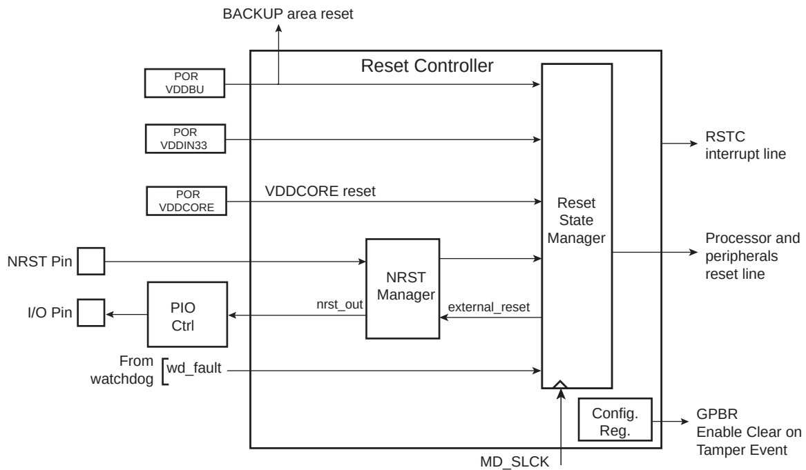
Figure 15-1. RSTC Block Diagram
