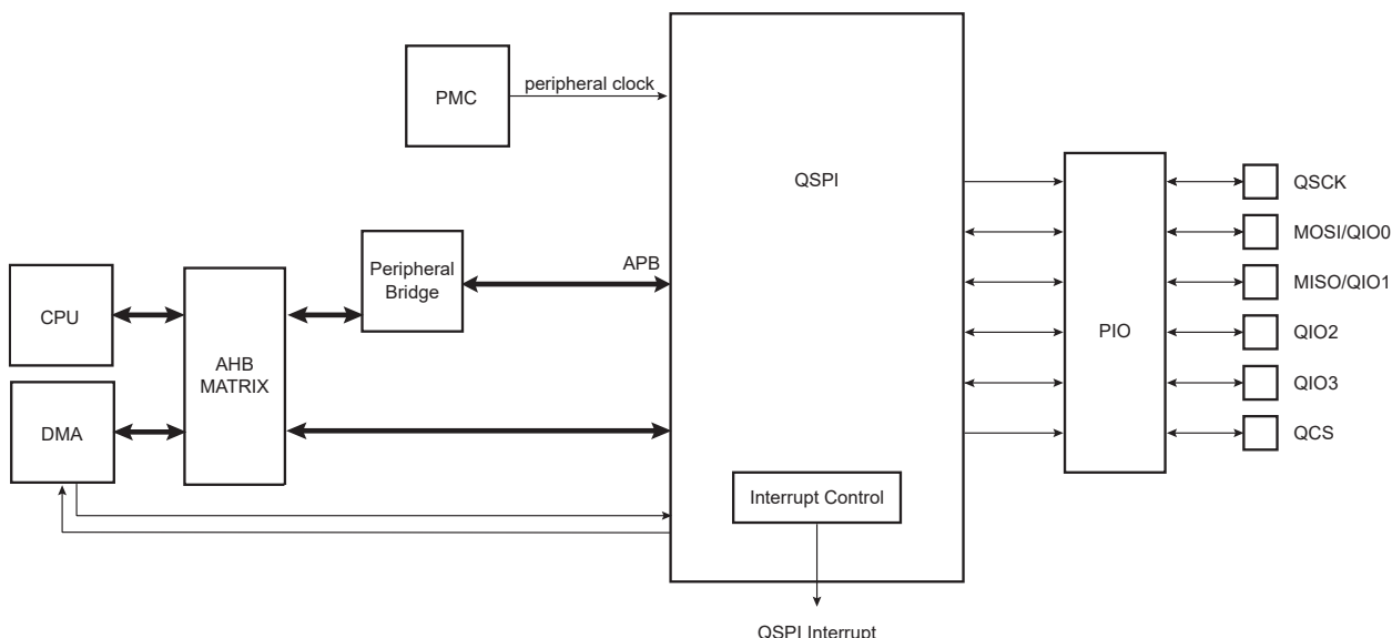
Figure 46-1. Block Diagram
