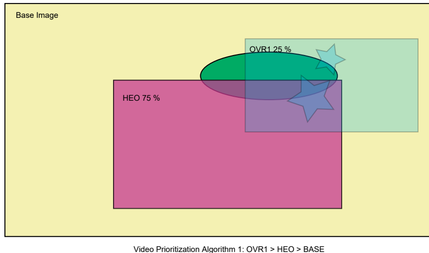
Figure 37-14. 256-level Alpha Blending
