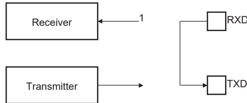
Figure 45-69. Remote Loopback Mode Configuration
