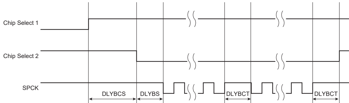
Figure 45-81. Programmable Delays
