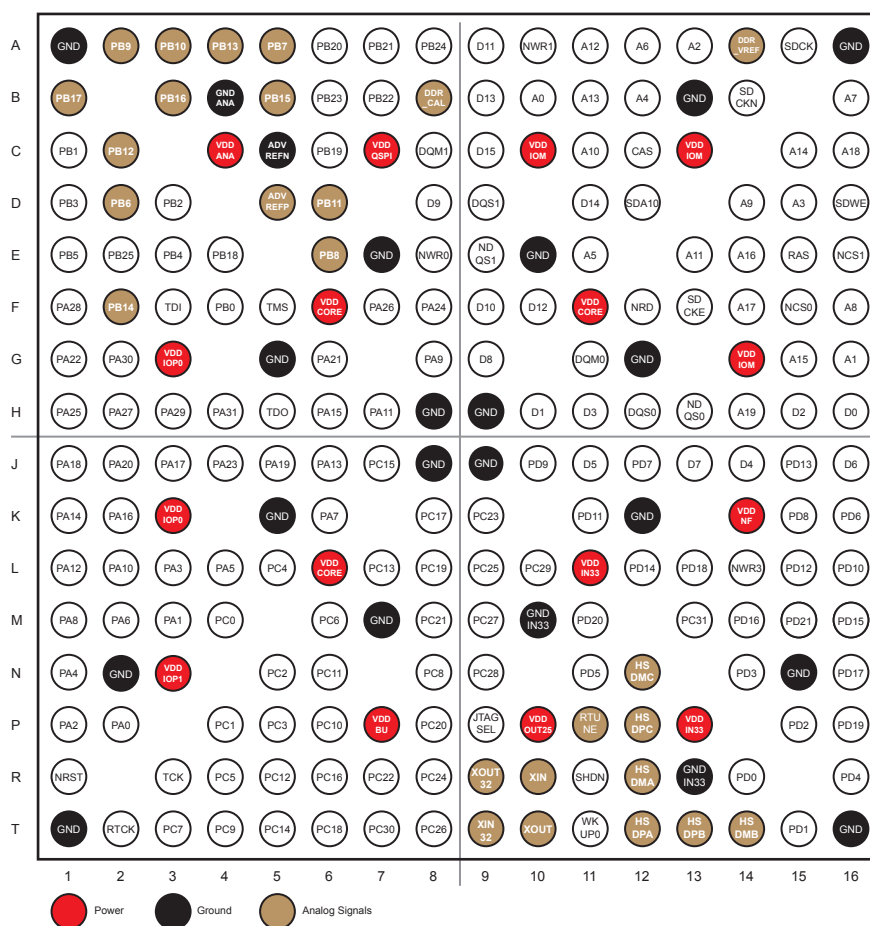
Figure 5-1. SAM9X60 BGA228 Pinout
