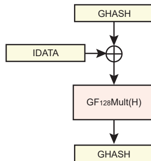
Figure 52-7. Single \text{GHASH}_H Block Diagram ( \text{AADLEN} \leq 0x10 and \text{CLEN} = 0 )
