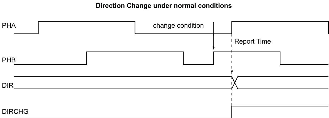
Figure 50-20. Rotation Change Detection
