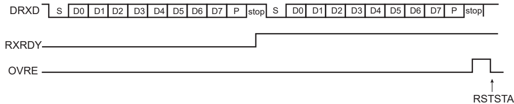
Figure 21-4. Character Reception
