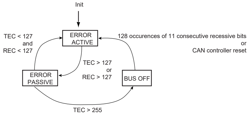
Figure 49-7. Line Error Mode
