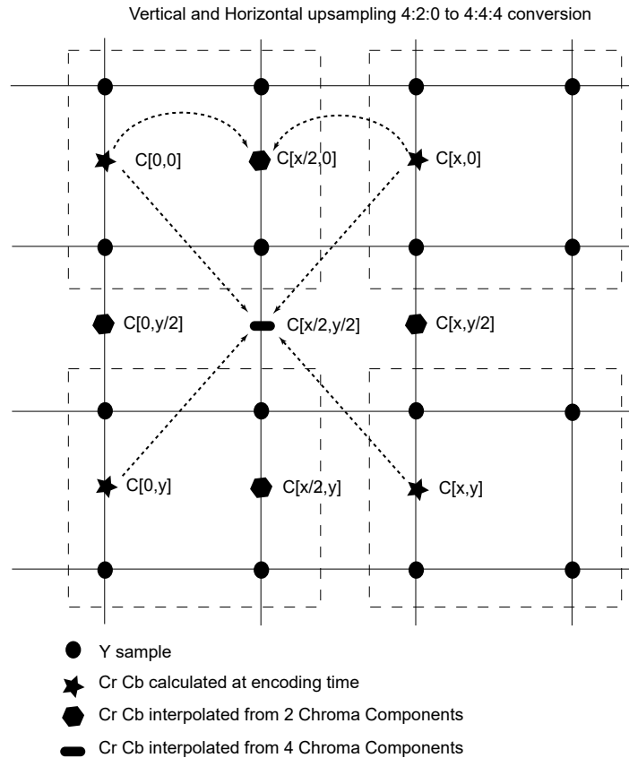
Figure 37-6. 4:2:0 Upsampling Algorithm
