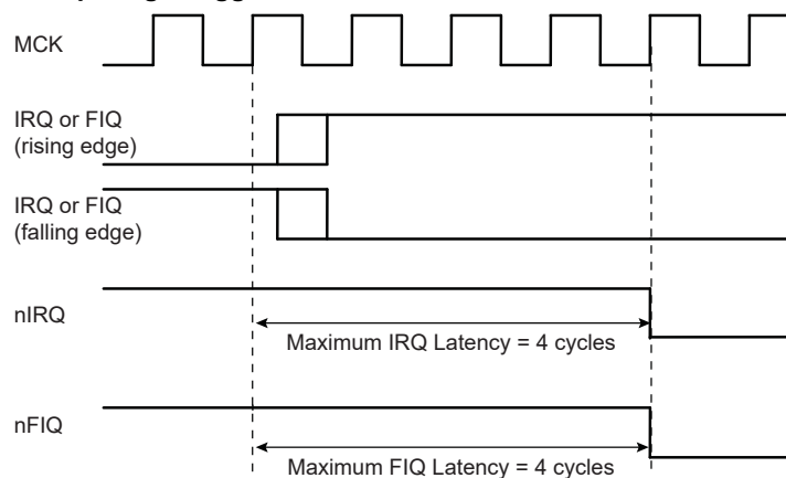
Figure 25-6. External Interrupt Edge Triggerged Source
