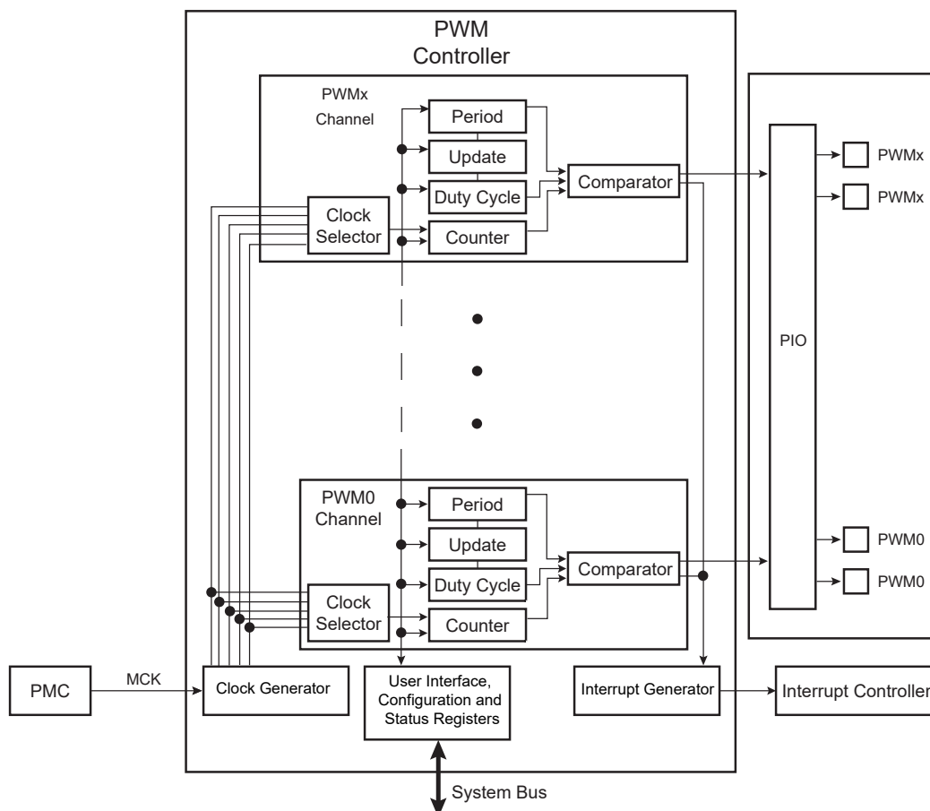
Figure 51-1. Pulse Width Modulation Controller Block Diagram
