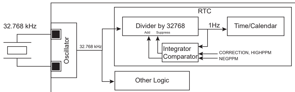
Figure 17-6. Calibration Circuitry
