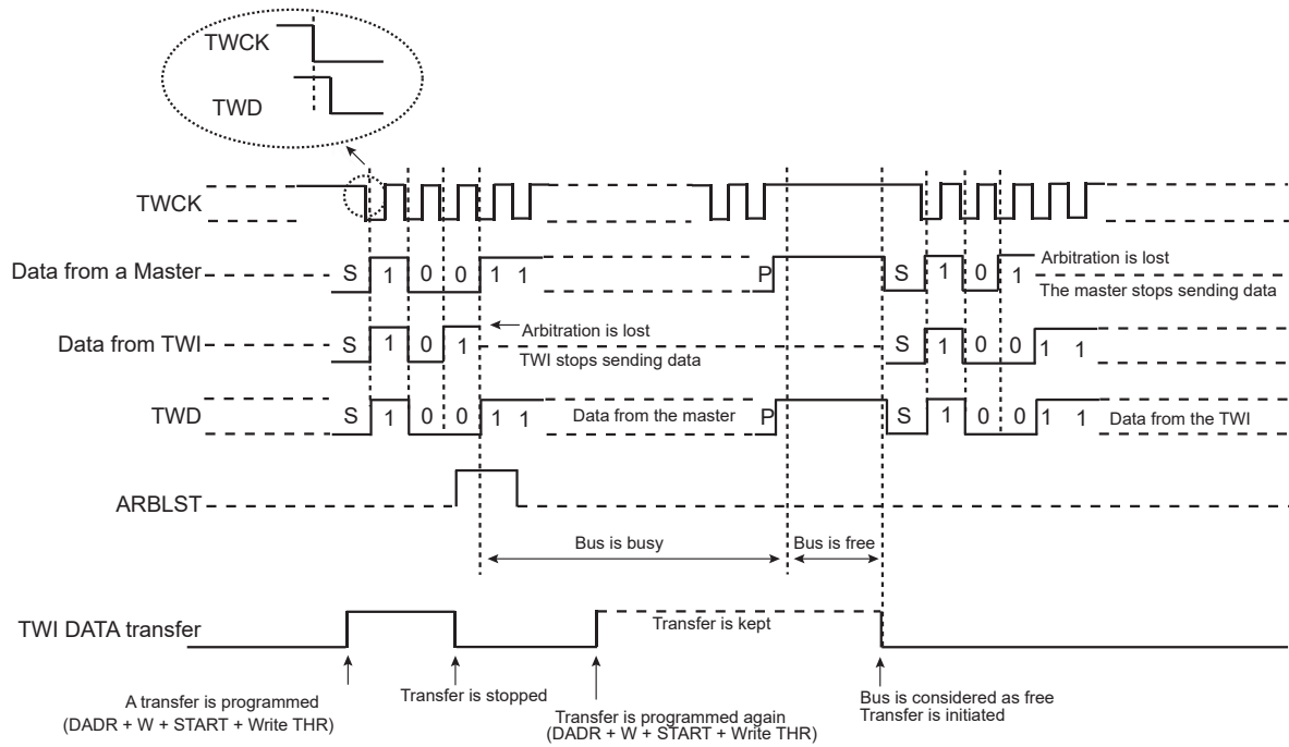
Figure 45-118. Arbitration Cases
