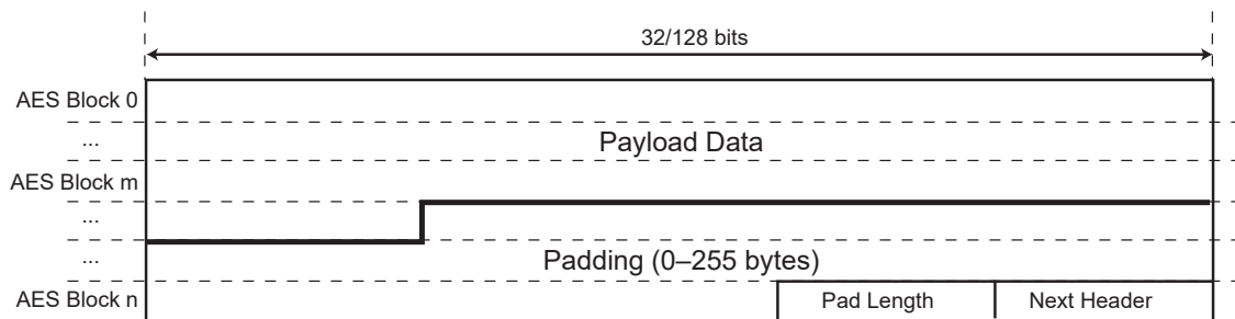
Figure 52-10. IPSEC Padding
