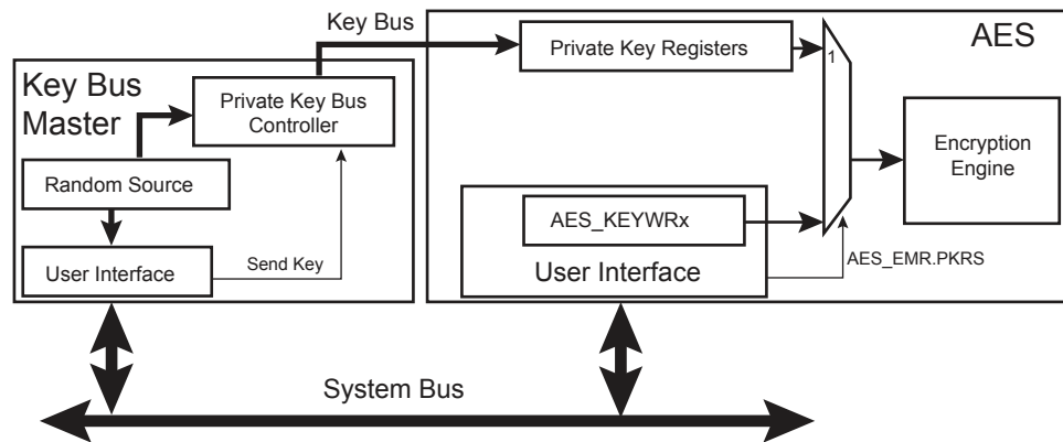
Figure 52-17. Key Selection
