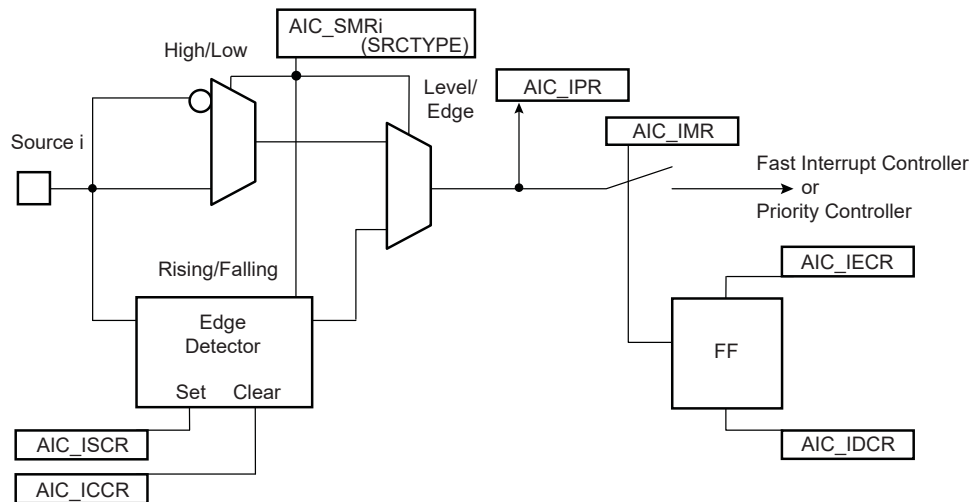
Figure 25-5. External Interrupt Source Input Stage
