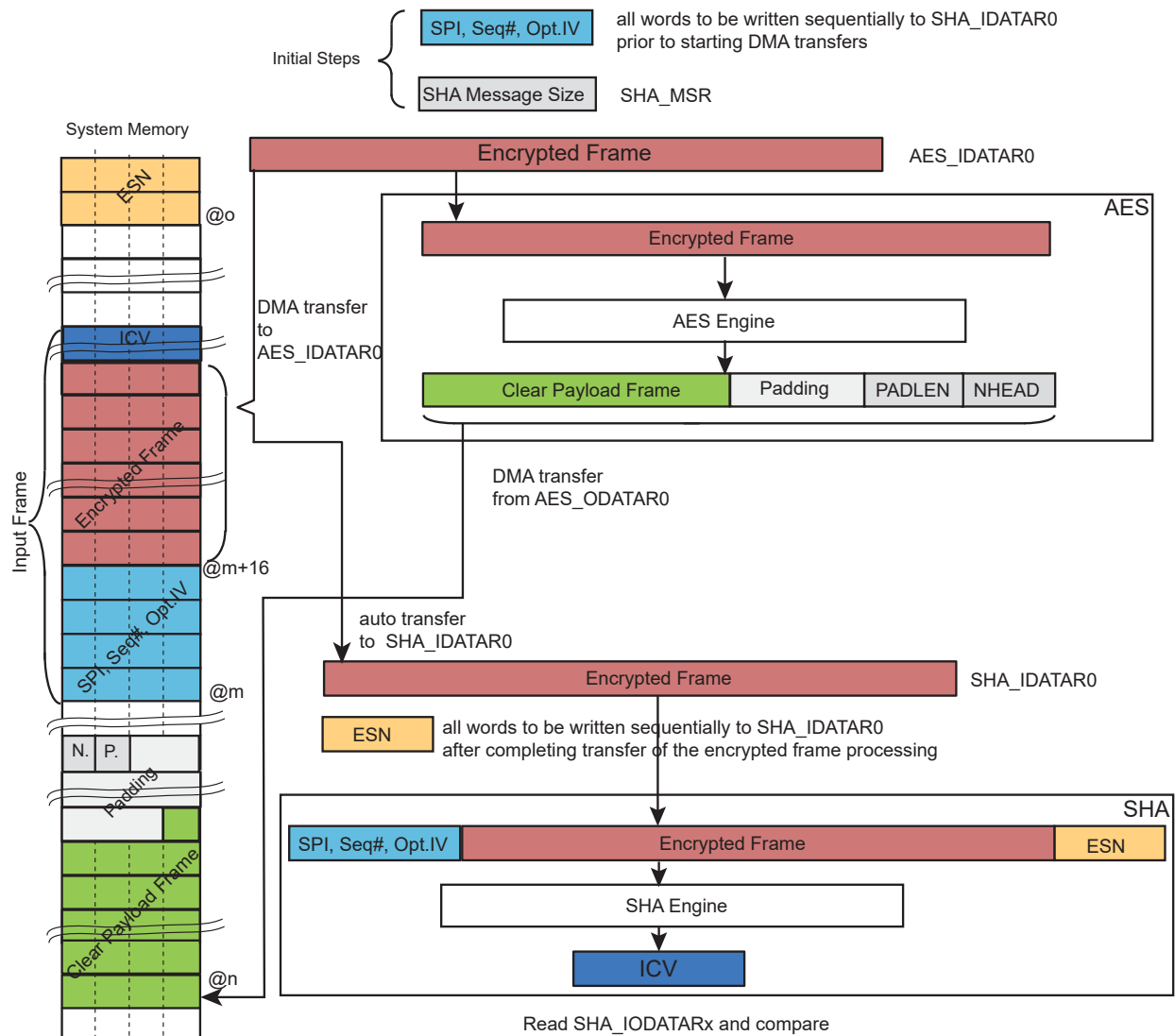
Figure 52-16. Decryption of an ESP IPsec Frame with ESN
