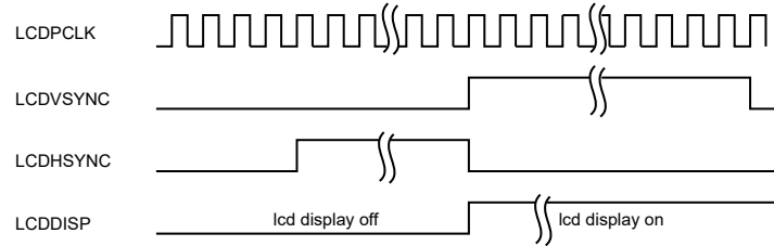
Figure 37-19. DISP Signal Timing Diagram
