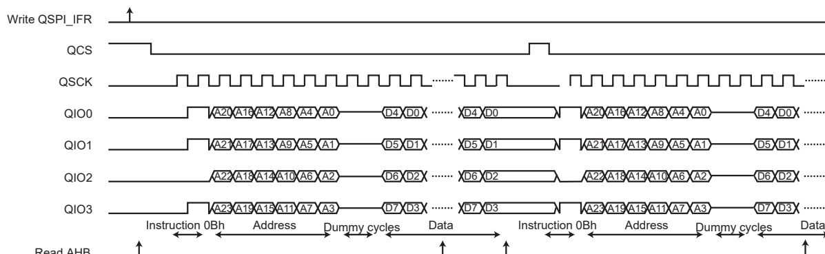
Figure 46-18. Instruction Transmission Waveform 8
