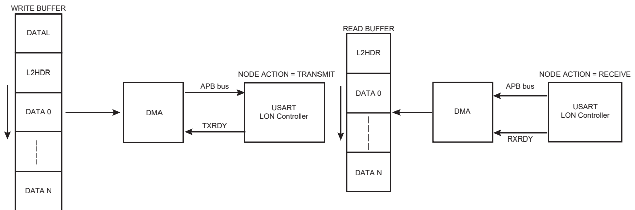
Figure 45-64. DMAM = 0
