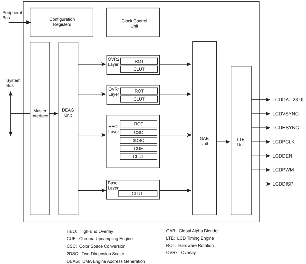
Figure 37-1. LCDC Block Diagram
