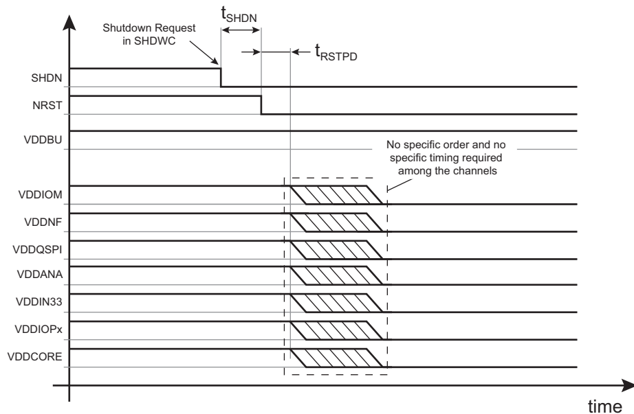
Figure 57-4. Recommended Power Sequence at Backup Mode Entry
