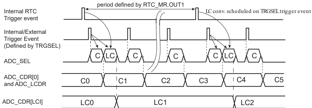
Figure 56-9. Independent Trigger Measurement for Last Channel (ADC_CHSR[LCI] = 0 and ADC_TRGR.TRGMOD = 1, 2, 3, 5)
