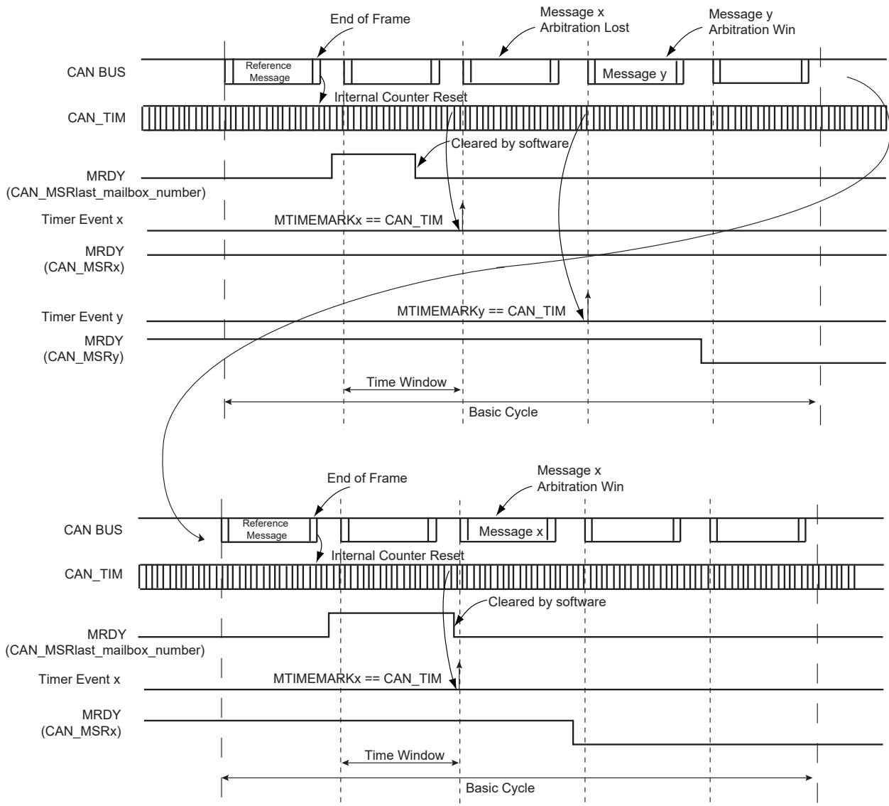
Figure 49-21. Time-Triggered Operations
