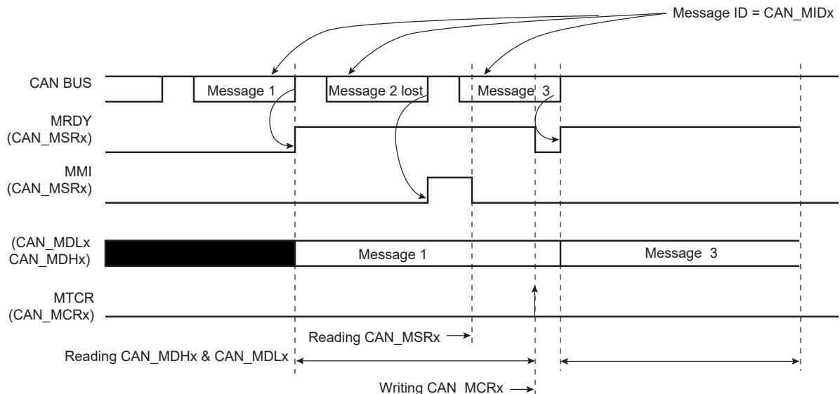
Figure 49-11. Receive Mailbox
