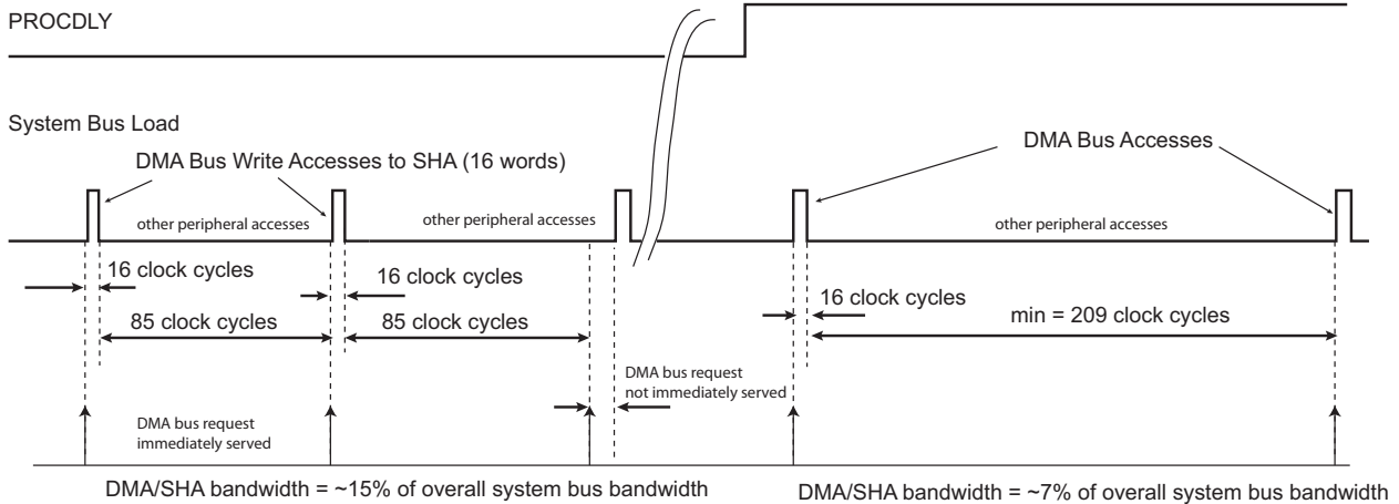
Figure 53-1. Bandwidth Usage in SHA-1 Mode
