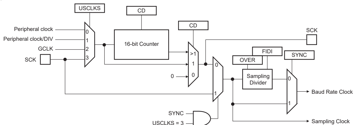
Figure 45-2. Baud Rate Generator
