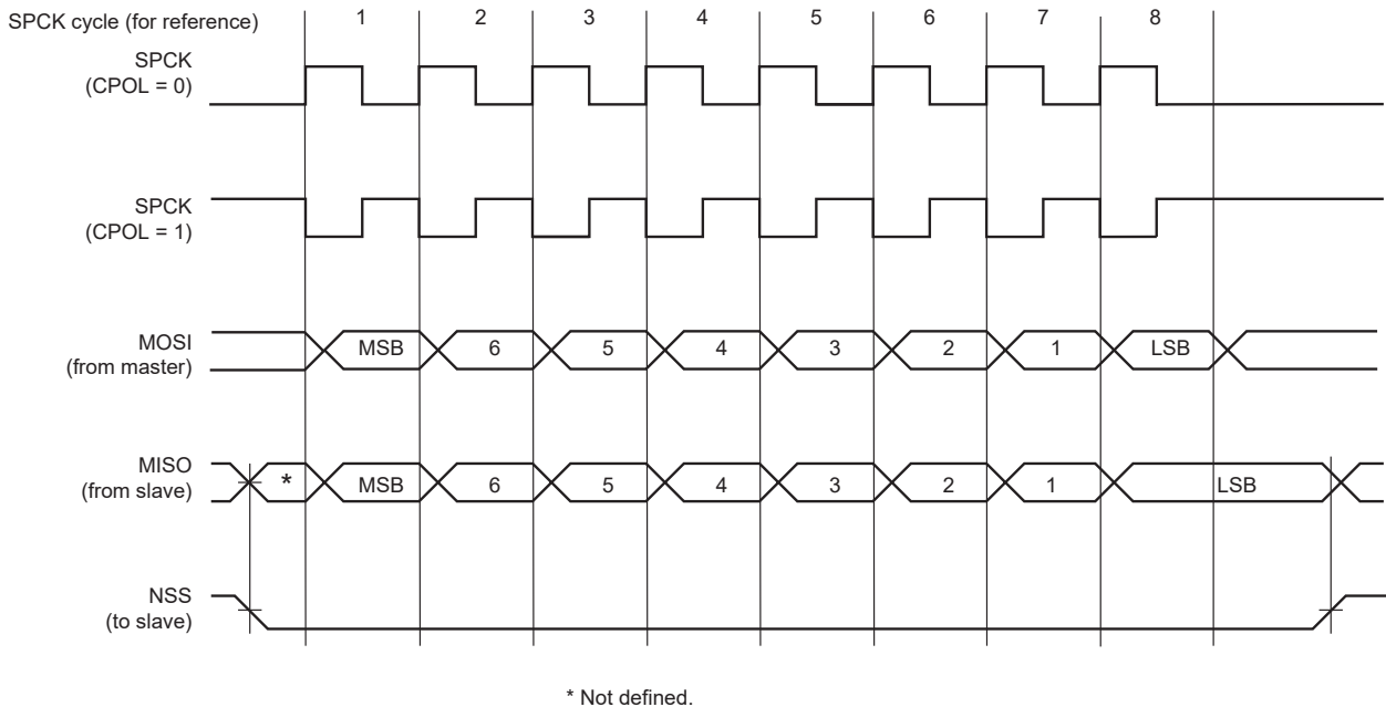
Figure 45-76. SPI Transfer Format (NCPHA = 0, 8 bits per transfer)
