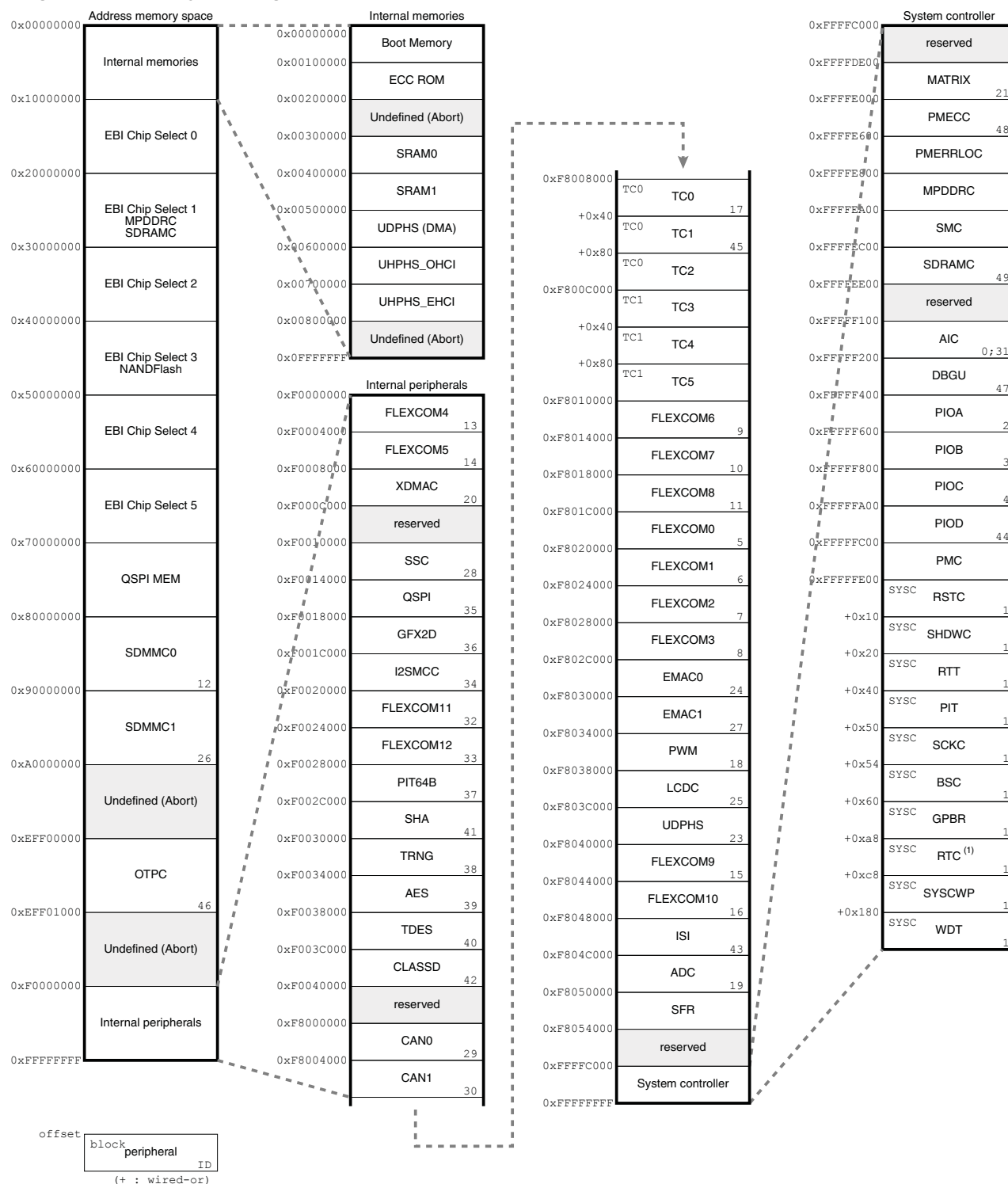
Figure 6-1. Memory Mapping
