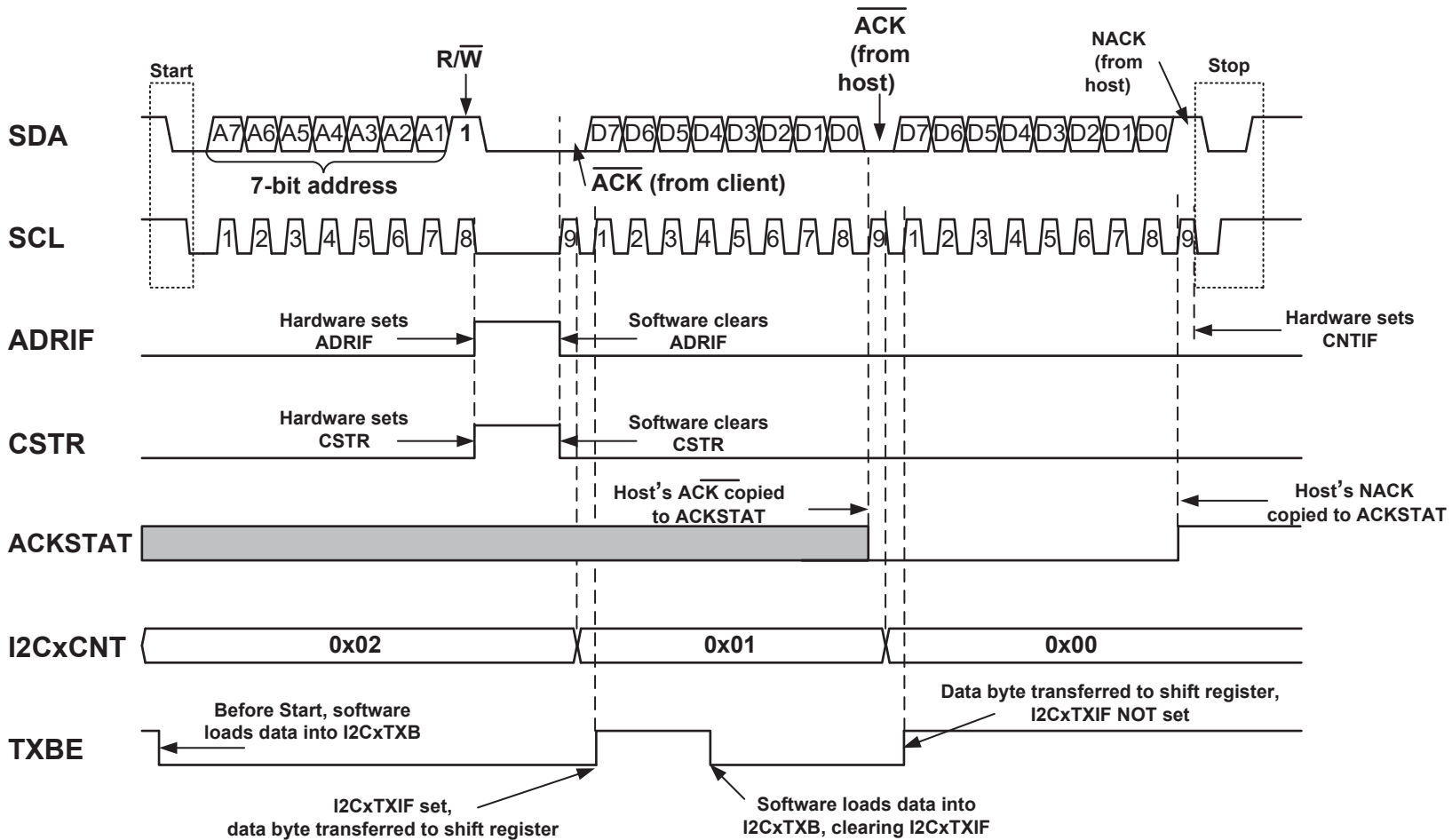
Figure 37-14. 7-Bit Client Mode Transmission (ADRIE = 1)
