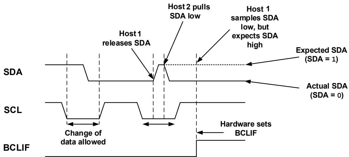
Figure 37-42. Bus Collision
