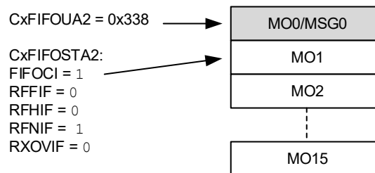
Figure 38-23. FIFO 2 - First Message Received
