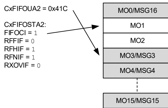
Figure 38-29. FIFO 2 - Two More Messages Read
