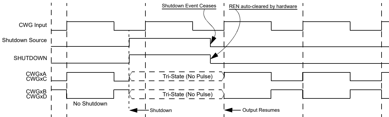
Figure 32-16. Shutdown Functionality, Auto-Restart Enabled (REN = 1, LSAC = 'b01, LSB0 = 'b01)
