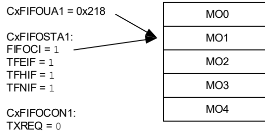
Figure 38-21. FIFO 1 - FIFO Fully Transmitted
