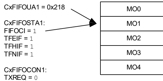
Figure 38-18. FIFO 1 - First Message Transmitted
