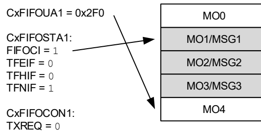
Figure 38-19. FIFO 1 - Three More Messages Loaded
