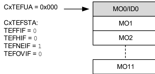
Figure 38-37. TEF - First Transmit Message is Stored
