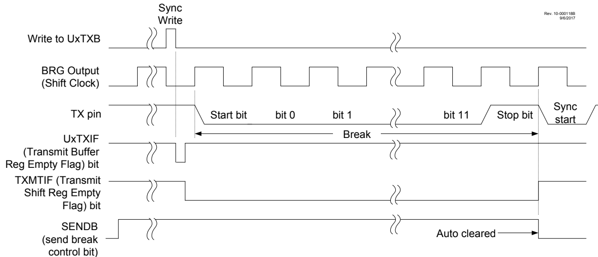
Figure 35-15. Send-Break Sequence
