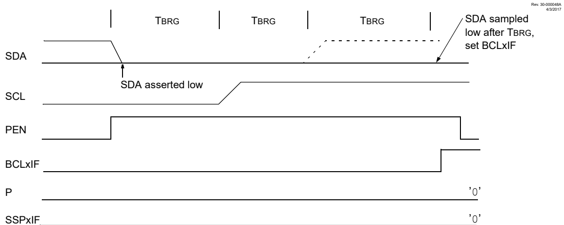
Figure 29-40. Bus Collision During a Stop Condition (Case 1)
