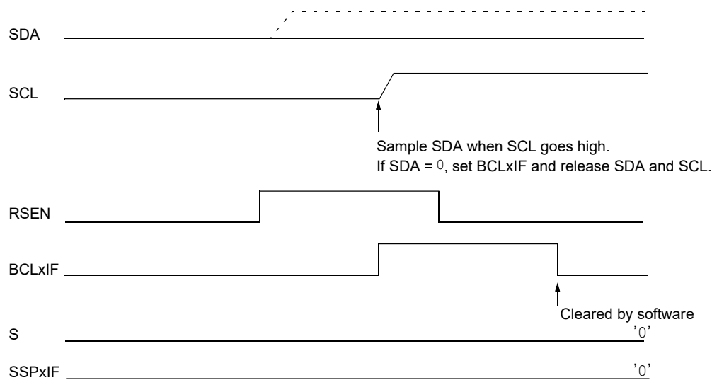
Figure 29-38. Bus Collision During a Repeated Start Condition (Case 1)
