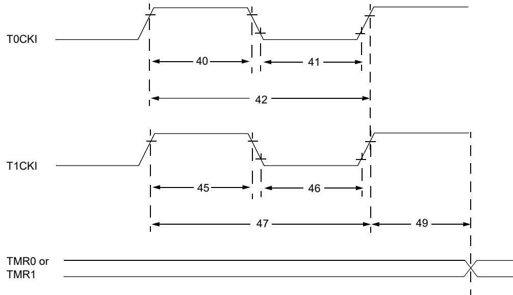
Figure 41-7. Timer0 and Timing1 External Clock Timings
