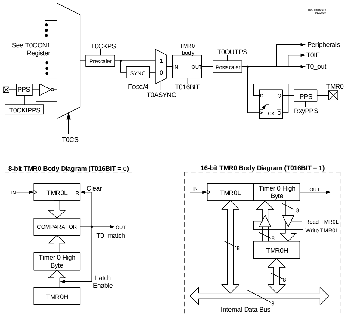
Figure 20-1. Timer0 Block Diagram
