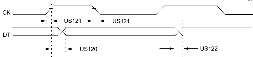
Figure 41-13. EUSART Synchronous Transmission (Host/Client) Timing
