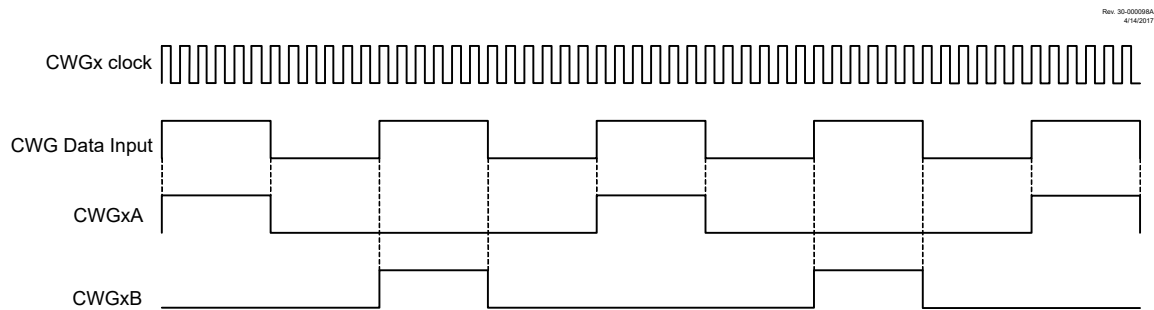
Figure 24-3. CWG Push-Pull Mode Operation
