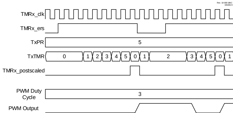
Figure 22-4. Hardware Gate Mode Timing Diagram (MODE = 'b000001)
