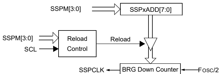
Figure 29-42. Baud Rate Generator Block Diagram
