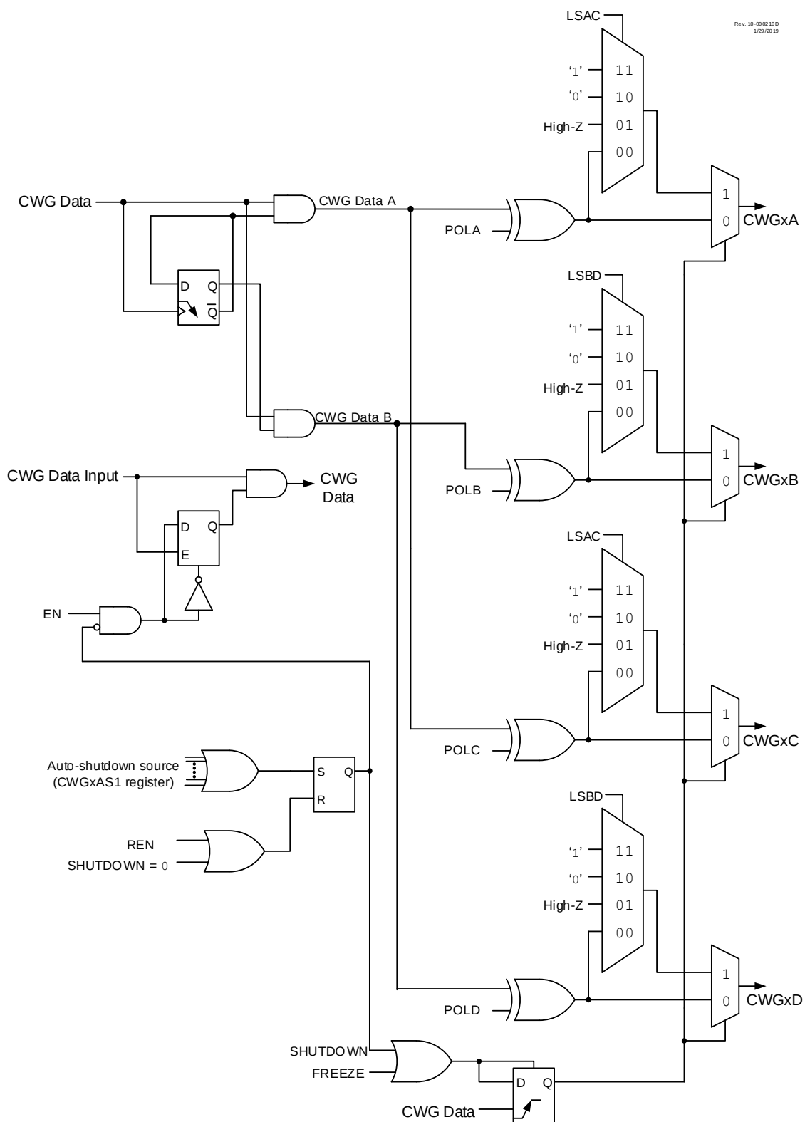
Figure 24-4. Simplified CWG Block Diagram (Push-Pull Mode, MODE = 'b101)
