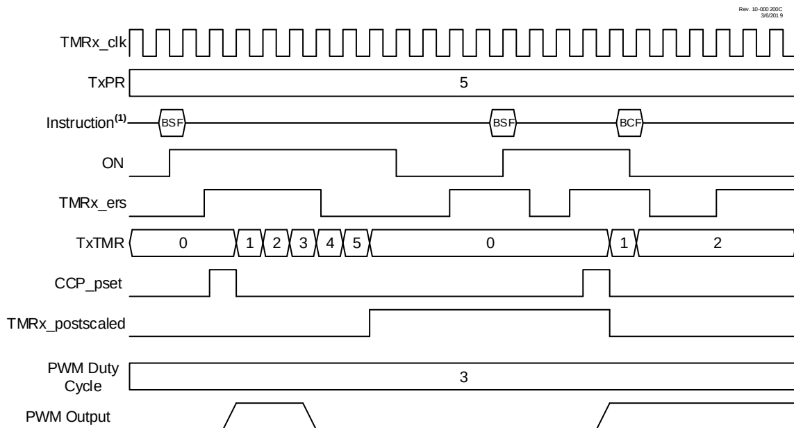
Figure 22-8. Edge Triggered One Shot Mode Timing Diagram (MODE = 'b01001)
