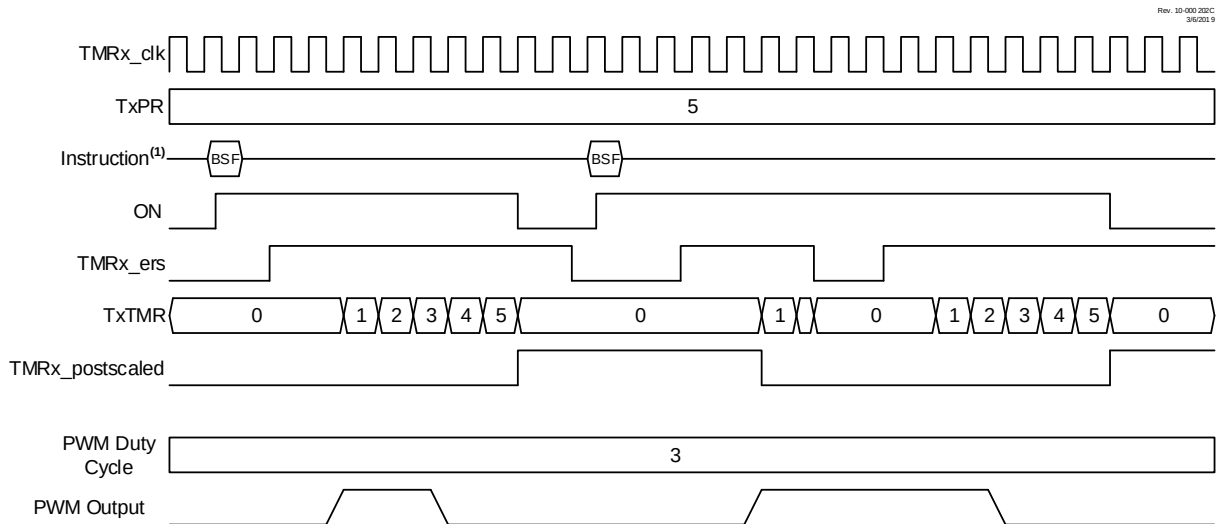
Figure 22-10. Low Level Reset, Edge Triggered Hardware Limit One Shot Mode Timing Diagram (MODE = 'b011110)
