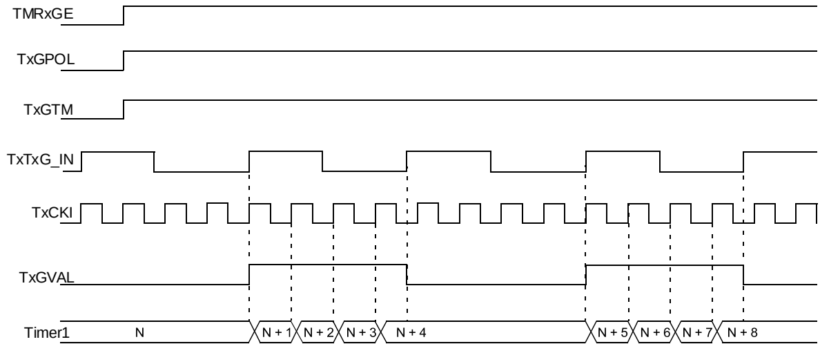
Figure 21-5. Timer1 Gate Toggle Mode
