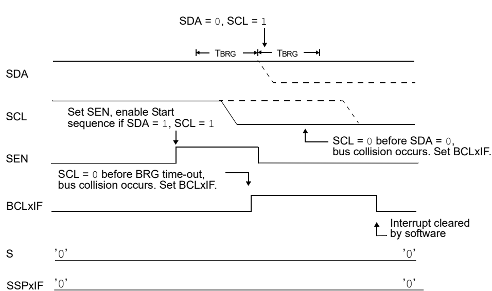
Figure 29-36. Bus Collision During Start Condition (SCL = 0)
