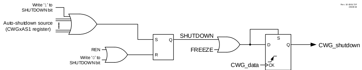
Figure 24-14. CWG Shutdown Block Diagram
