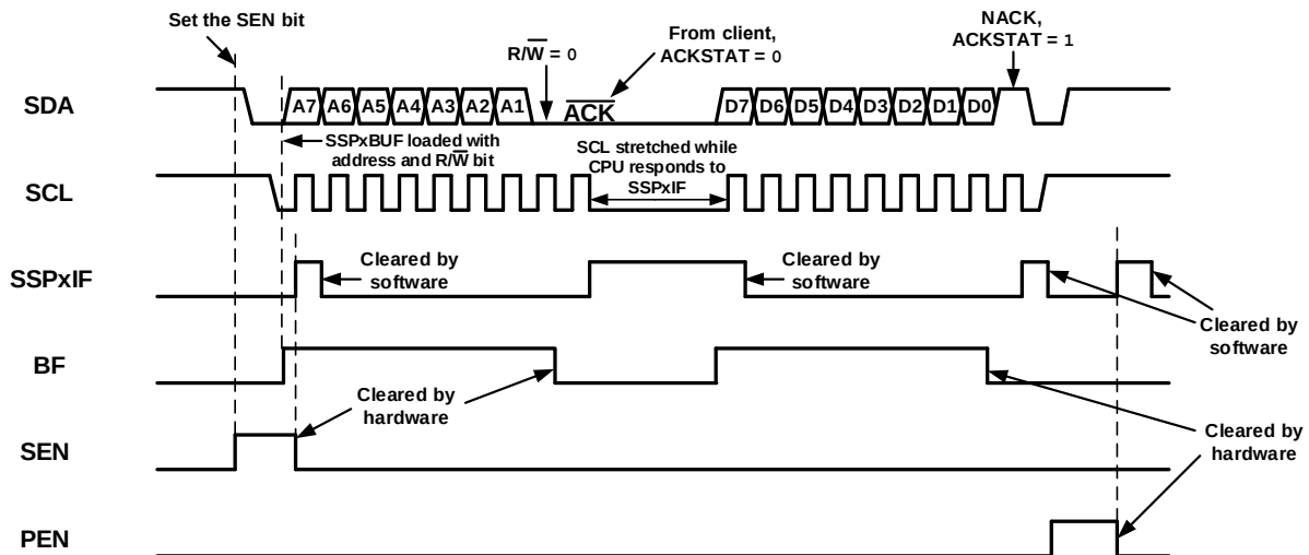
Figure 29-30. I 2 C Host Mode Waveform (Transmission, 7-Bit Address)
