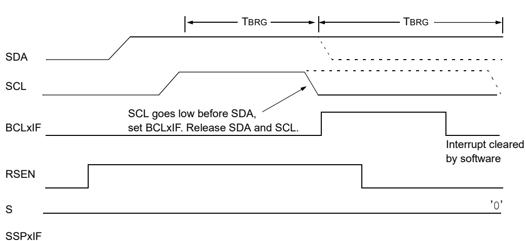
Figure 29-39. Bus Collision During Repeated Start Condition (Case 2)
