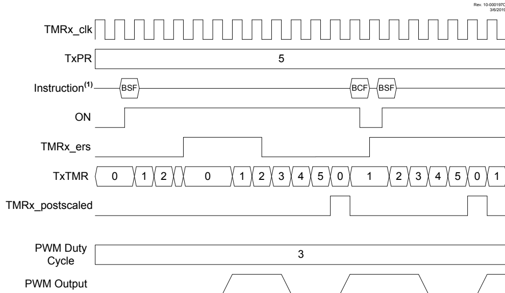
Figure 22-5. Edge Triggered Hardware Limit Mode Timing Diagram (MODE = 'b00100)
