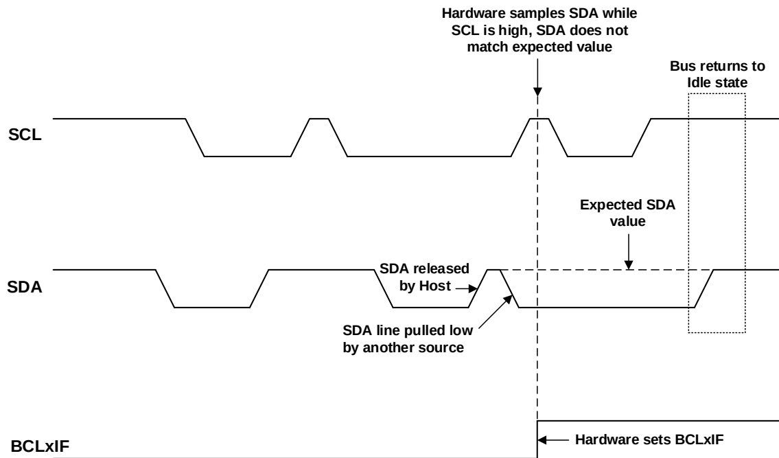
Figure 29-34. Bus Collision Timing for Transmit and Acknowledge
