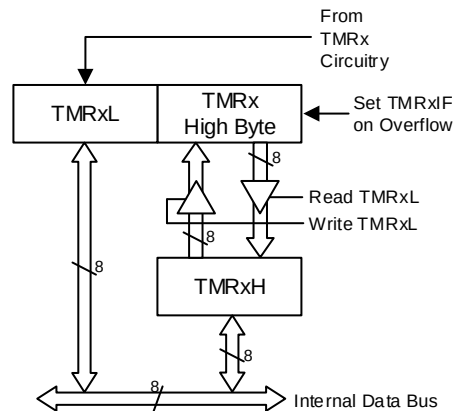
Figure 21-3. Timer1 16-Bit Read/Write Mode Block Diagram
