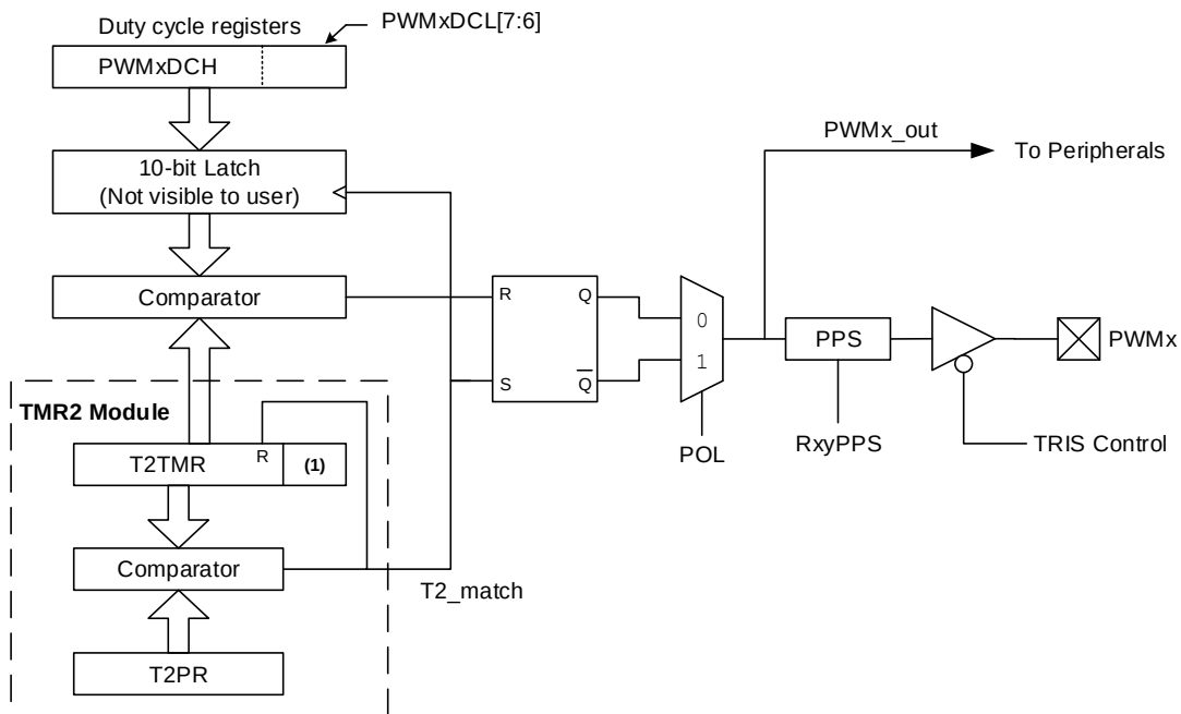
Figure 27-1. Simplified PWM Block Diagram
