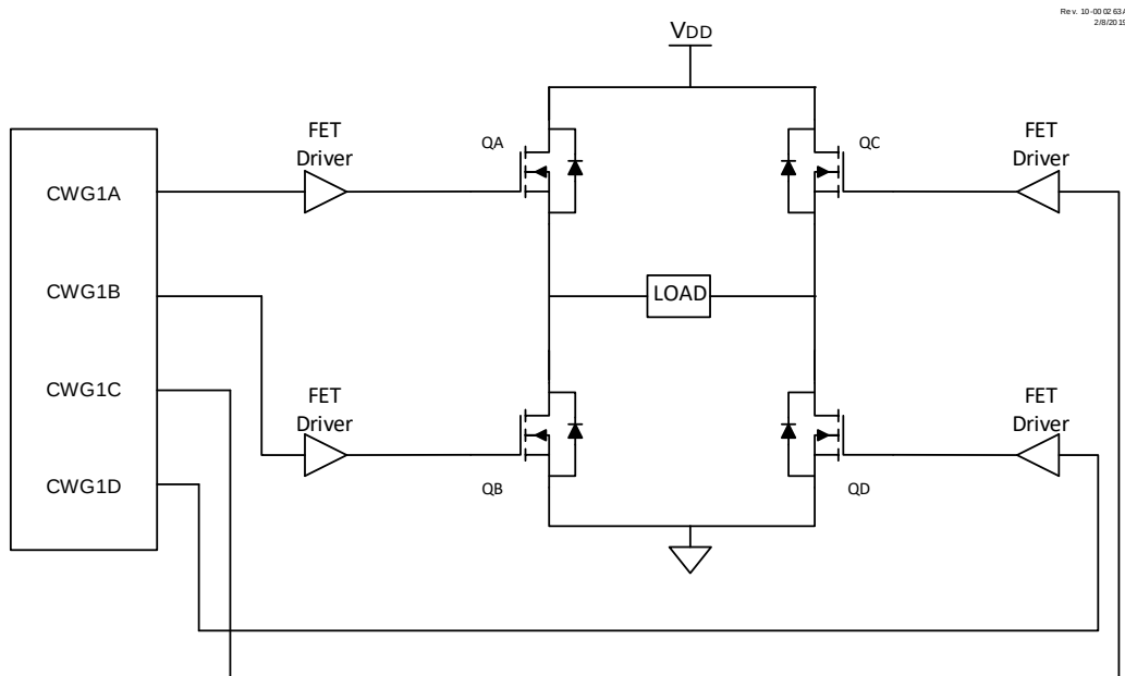
Figure 24-5. Example of Full-Bridge Application
