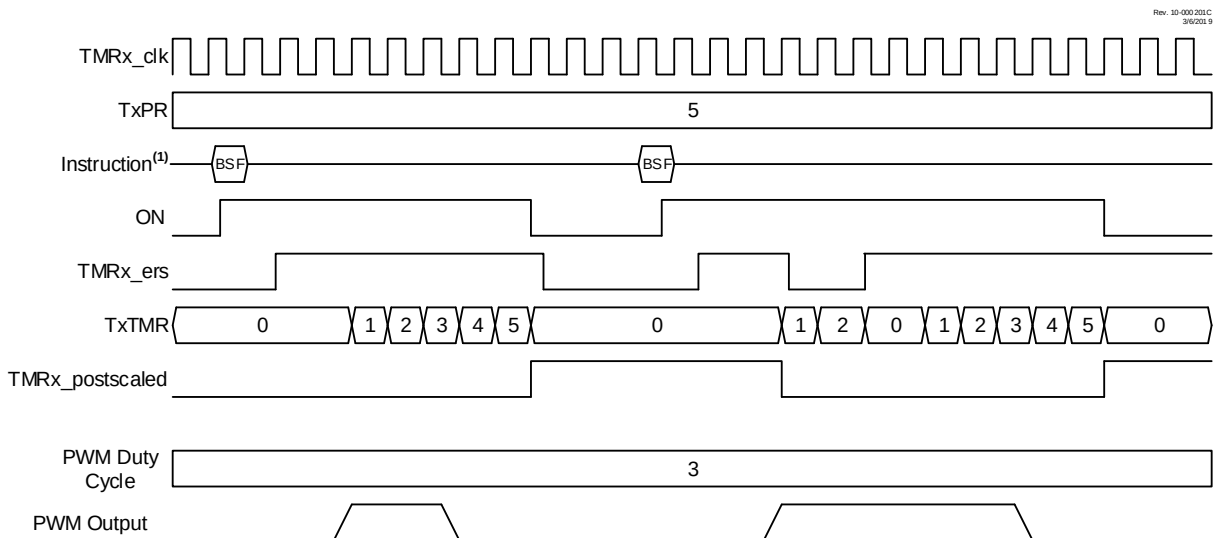
Figure 22-9. Edge Triggered Hardware Limit One Shot Mode Timing Diagram (MODE = 'b01100)
