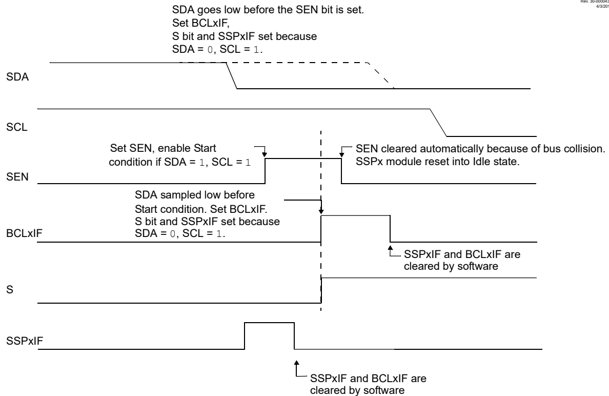
Figure 29-35. Bus Collision During Start Condition (SDA Only)
