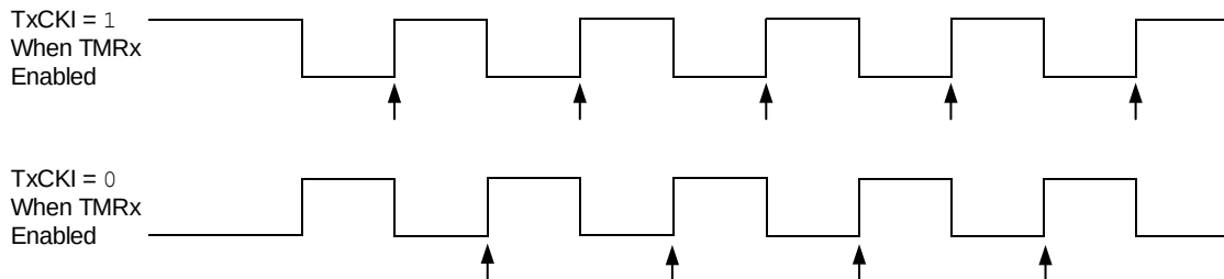
Figure 21-2. Timer1 Incrementing Edge
