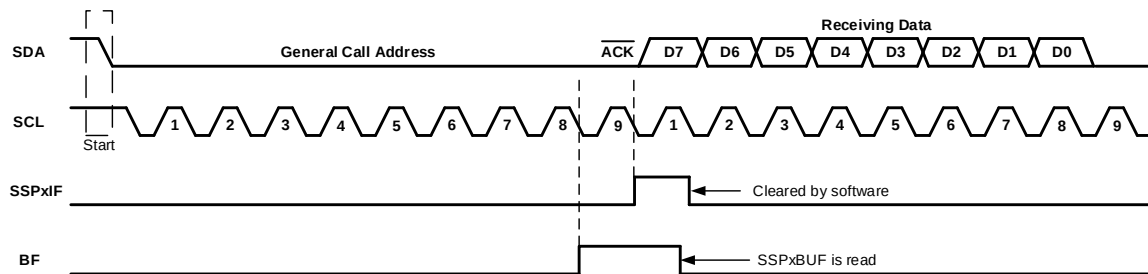
Figure 29-15. Client Mode General Call Address Sequence
