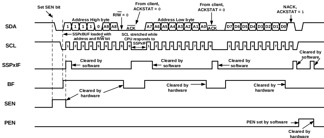
Figure 29-31. I 2 C Host Mode Waveform (Transmission, 10-Bit Address)
