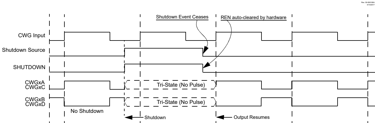
Figure 24-16. Shutdown Functionality, Auto-Restart Enabled (REN = 1, LSAC = 'b01, LSB0 = 'b01)
