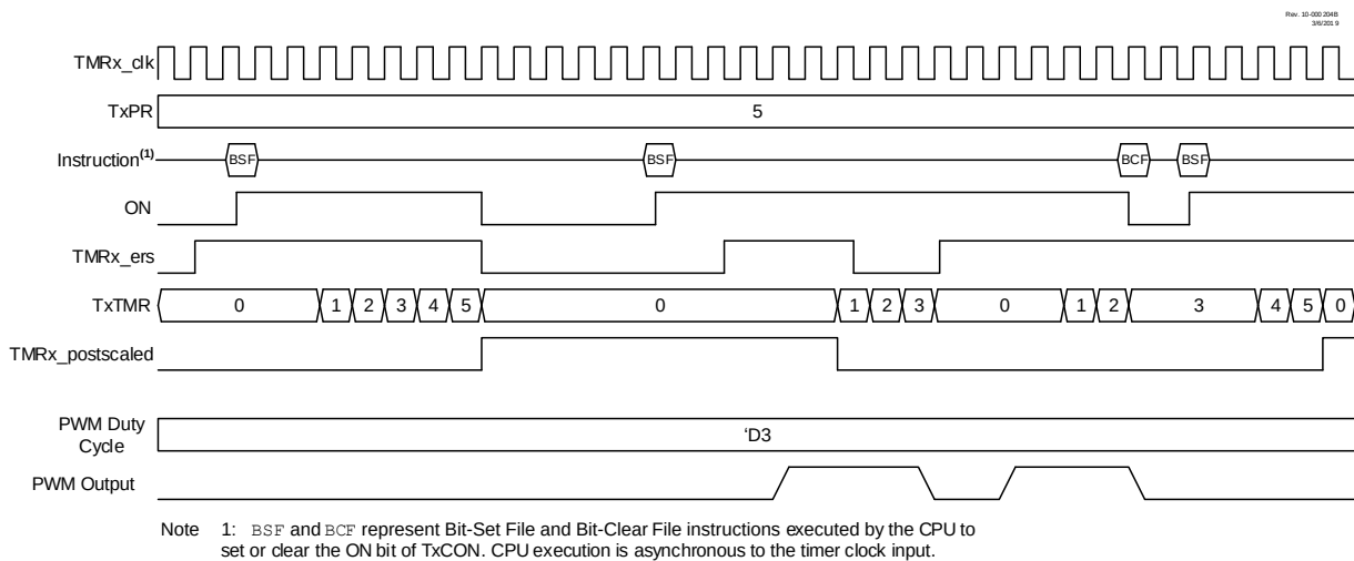
Figure 22-12. Level Triggered Hardware Limit One Shot Mode Timing Diagram (MODE = 'b10110)
