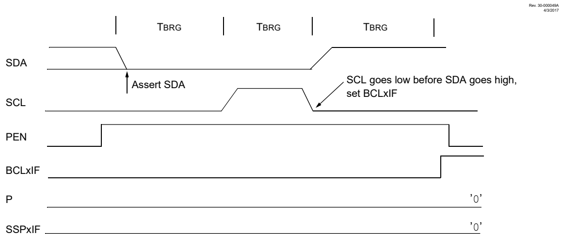
Figure 29-41. Bus Collision During a Stop Condition (Case 2)
