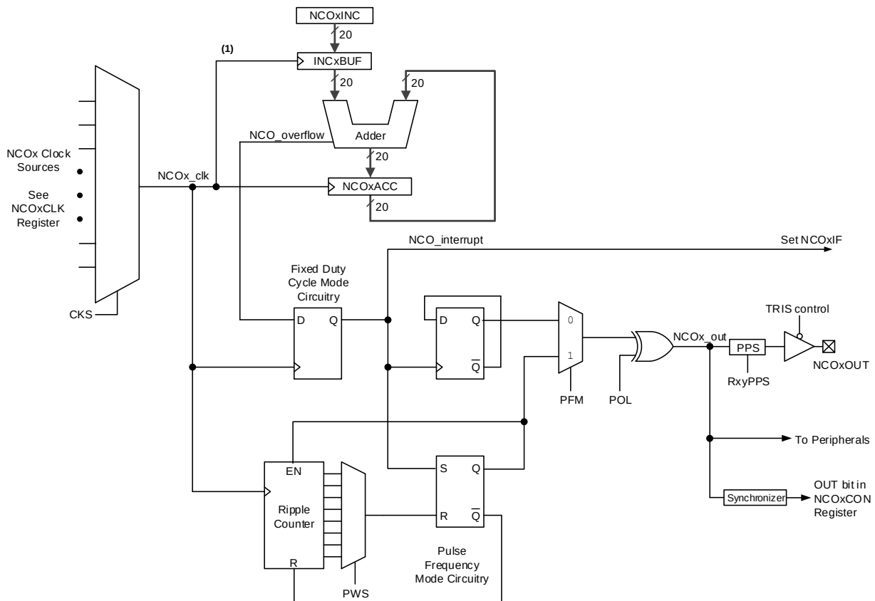
Figure 23-1. Numerically Controlled Oscillator Module Simplified Block Diagram
