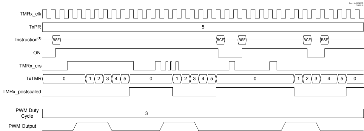
Figure 22-11. Rising Edge Triggered Monostable Mode Timing Diagram (MODE = 'b10001)
