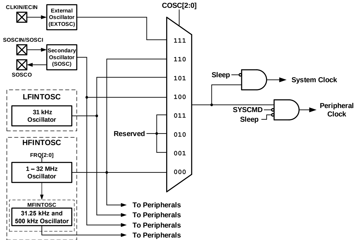
Figure 11-1. Clock Source Block Diagram
