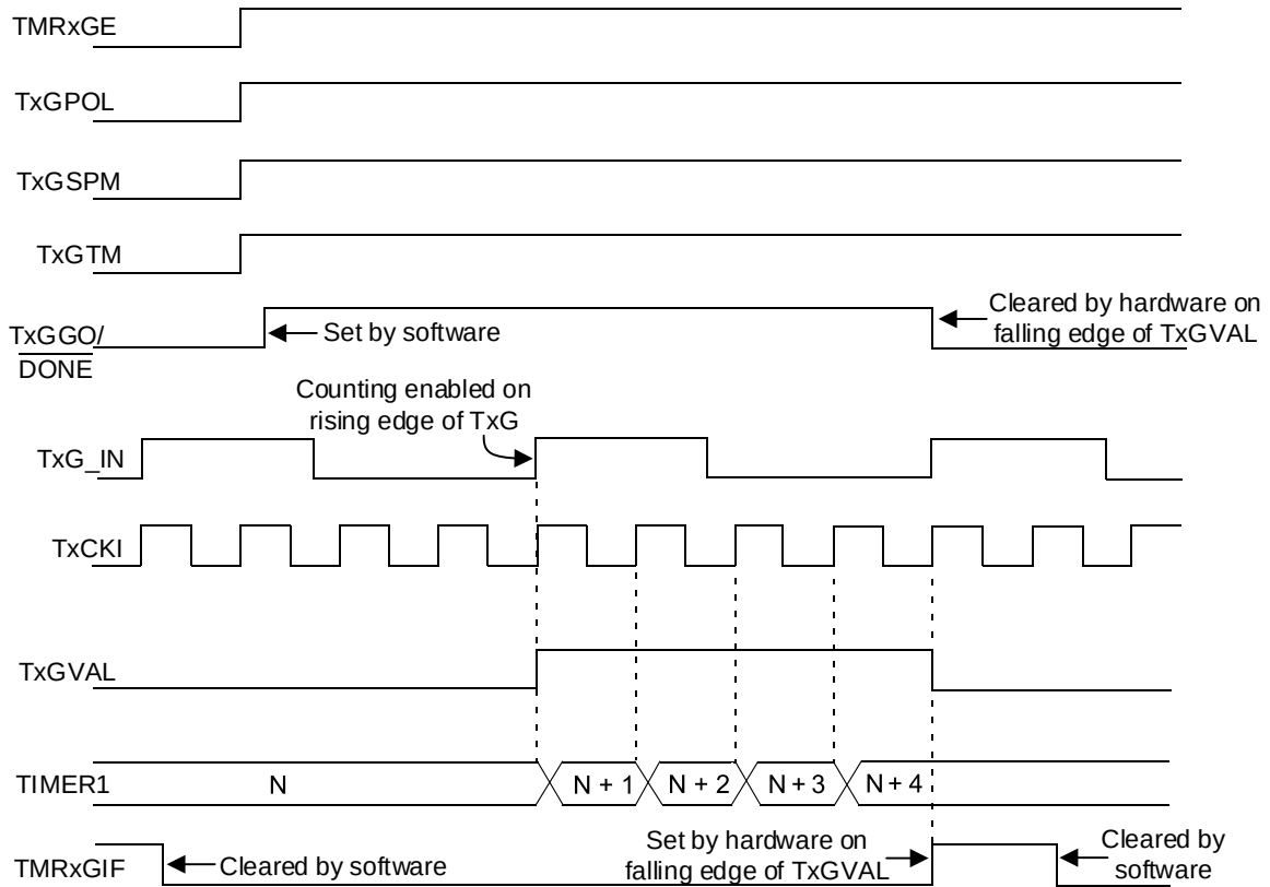
Figure 21-7. Timer1 Gate Single Pulse and Toggle Combined Mode
