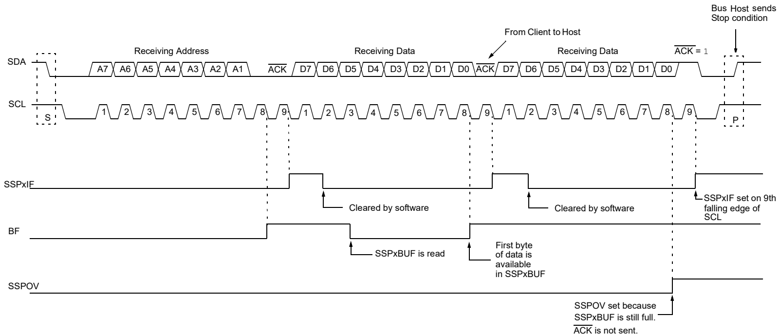
Figure 29-16. I 2 C Client, 7-Bit Address, Reception (SEN = 0, AHEN = 0, DHEN = 0)
