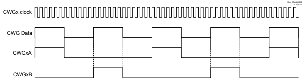
Figure 24-10. Example of Synchronous Steering (MODE = 'b001)
