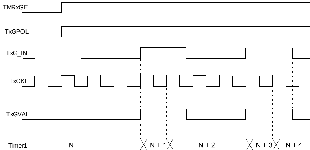
Figure 21-4. Timer1 Gate Enable Mode
