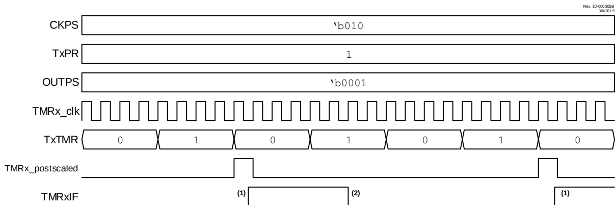
Figure 22-2. Timer2 Prescaler, Postscaler, and Interrupt Timing Diagram
