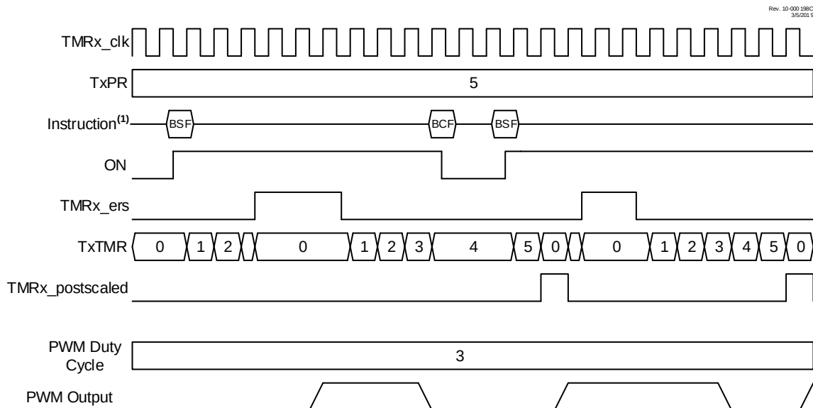
Figure 22-6. Level Triggered Hardware Limit Mode Timing Diagram (MODE = 'b00111)
