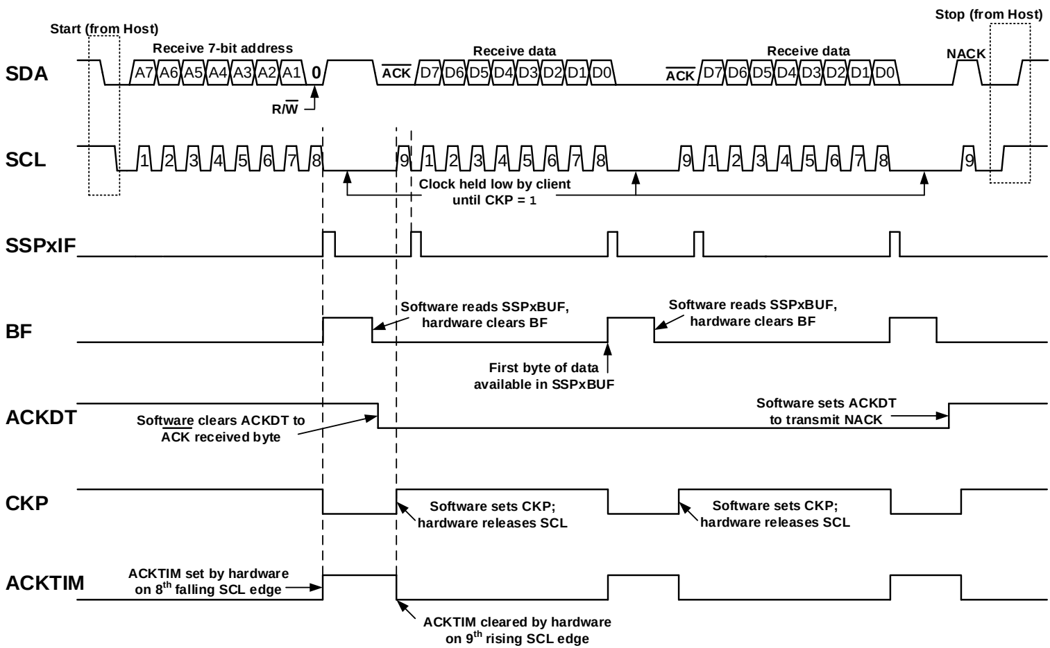
Figure 29-18. I 2 C Client, 7-Bit Address, Reception (SEN = 0, AHEN = 1, DHEN = 1)
