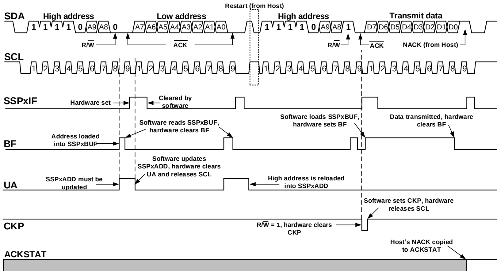
Figure 29-22. I 2 C Client, 10-Bit Address, Transmission (SEN = 0, AHEN = 0, DHEN = 0)
