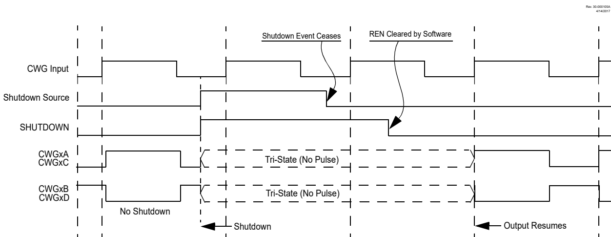
Figure 24-15. Shutdown Functionality, Auto-Restart Disabled ( REN = 0, LSAC = 'b01, LSBD = 'b01)
