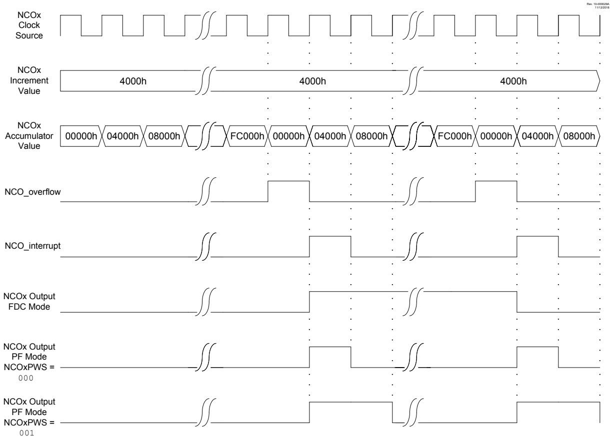
Figure 23-2. FDC Output Mode Timing Diagram
