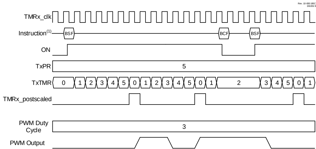
Figure 22-3. Software Gate Mode Timing Diagram (MODE = 'b00000)
