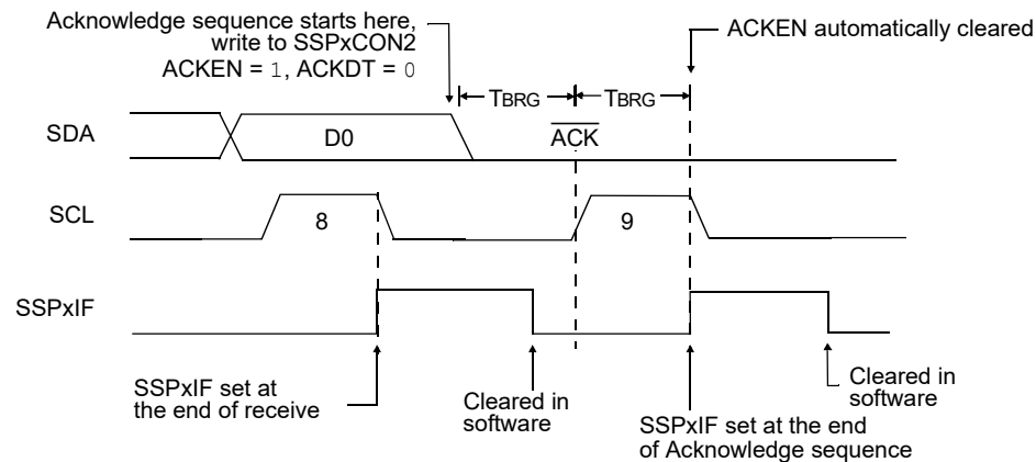
Figure 29-28. Acknowledge Sequence Waveform
