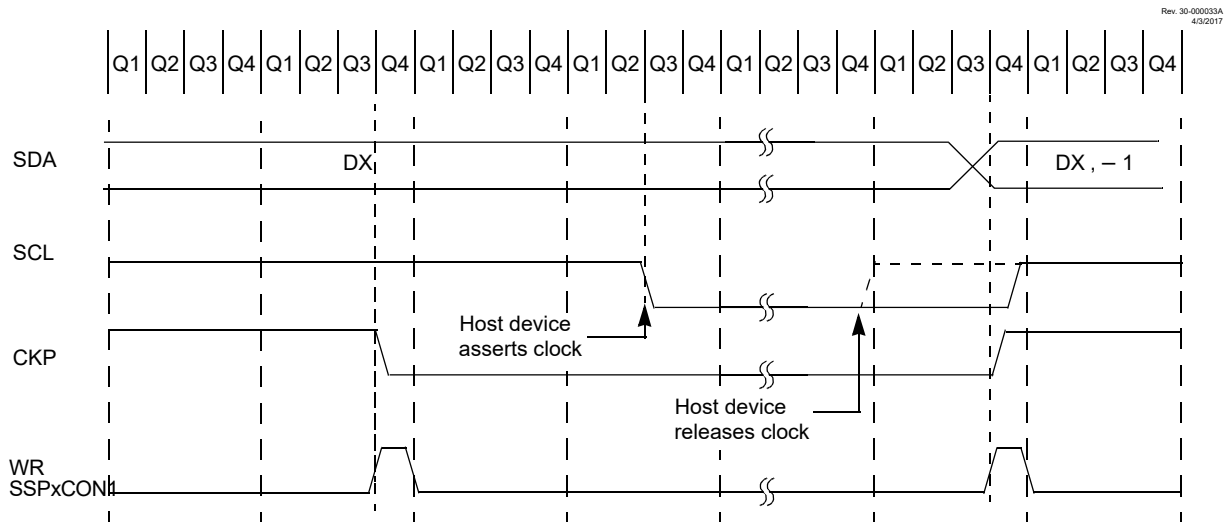
Figure 29-14. Clock Synchronization Timing
