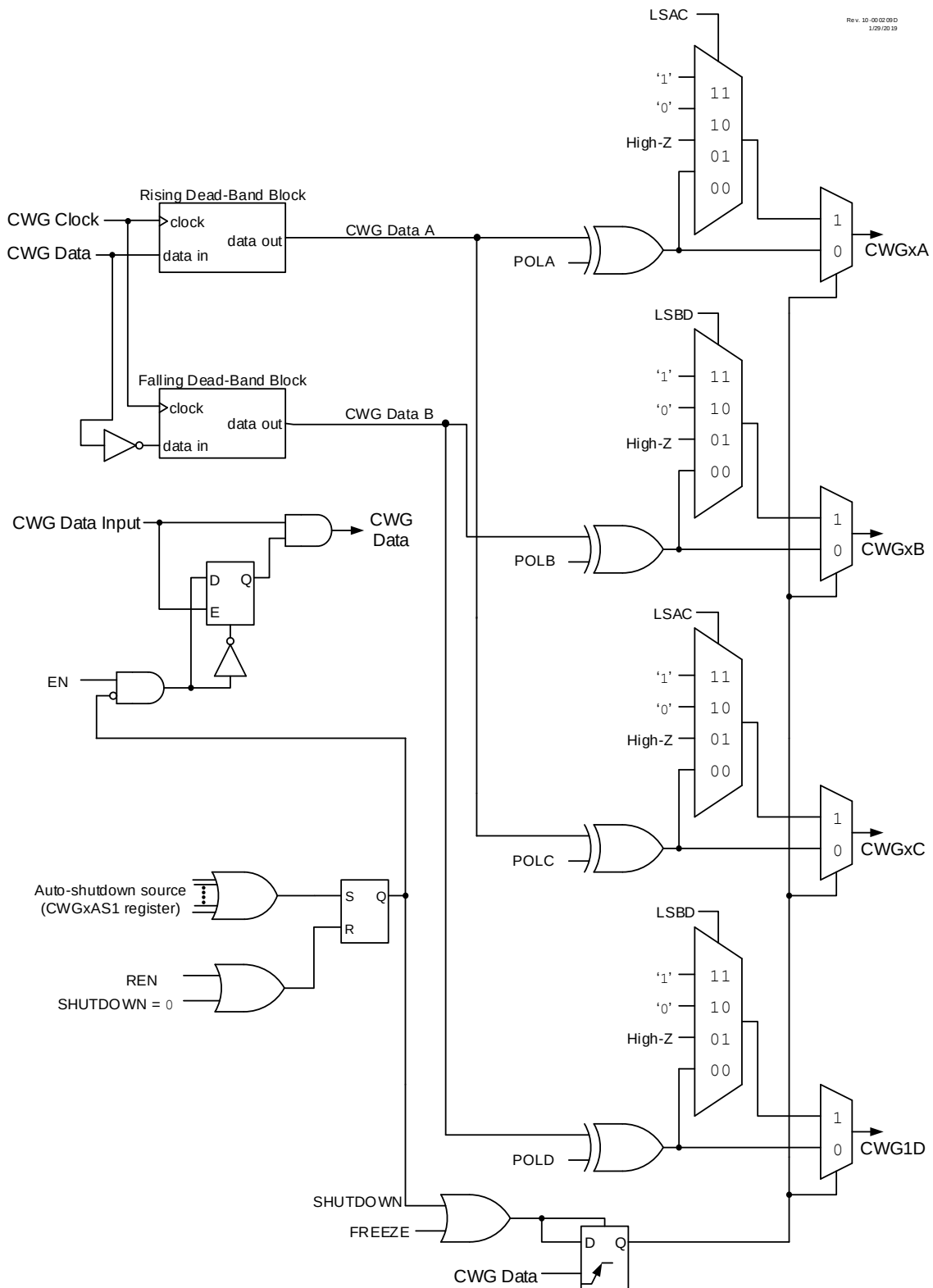
Figure 24-2. Simplified CWG Block Diagram (Half Bridge Mode, MODE = 'b100)
