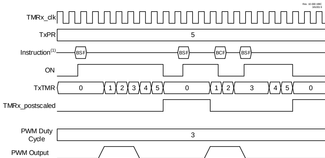
Figure 22-7. Software Start One Shot Mode Timing Diagram (MODE = 'b01000)
