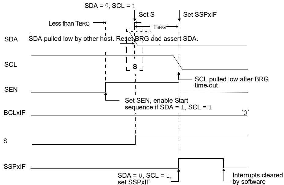
Figure 29-37. BRG Reset Due to SDA Arbitration During Start Condition
