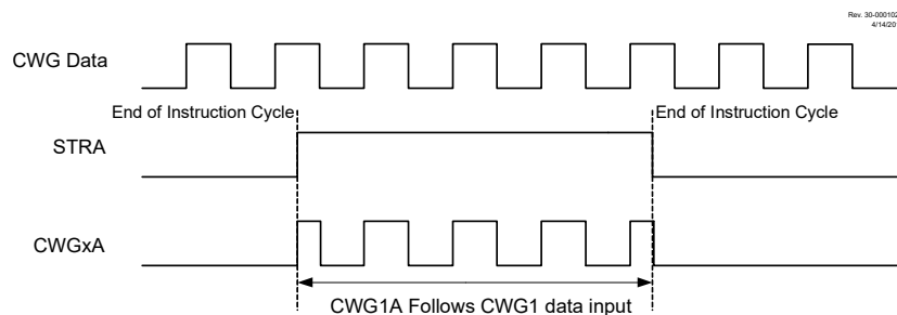
Figure 24-11. Example of Asynchronous Steering (MODE = 'b000)
