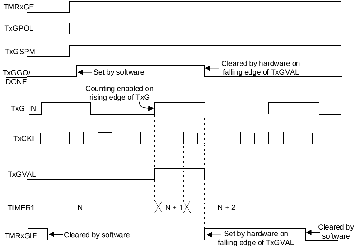
Figure 21-6. Timer1 Gate Single Pulse Mode
