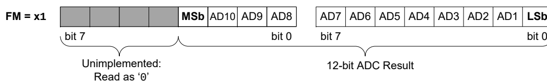
Figure 35-4. 12-bit ADC Conversion Result Alignment/Format: IC = 0, FM = x1
