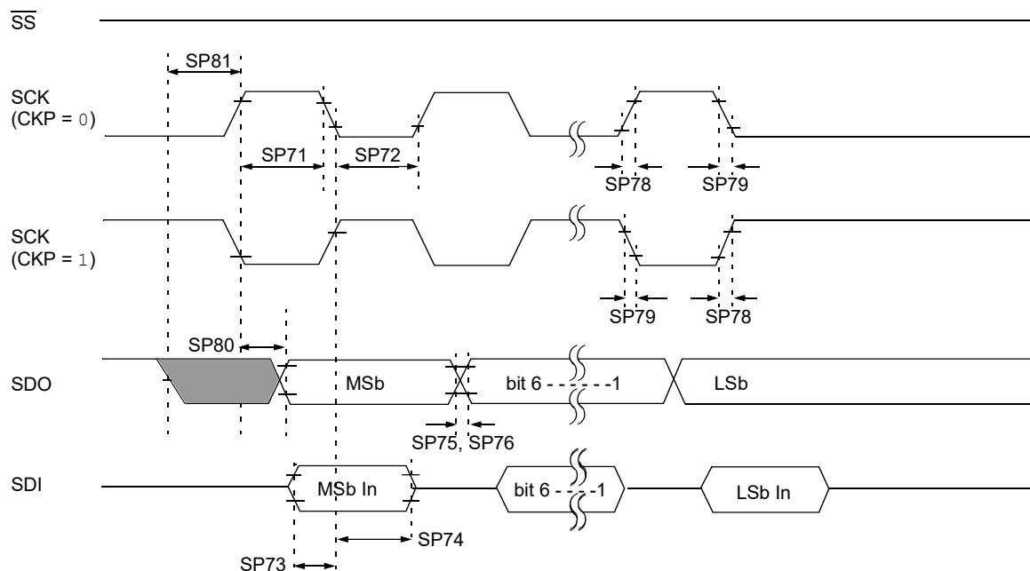
Figure 48-15. SPI Host Mode Timing (CKE = 0, SMP = 0)
