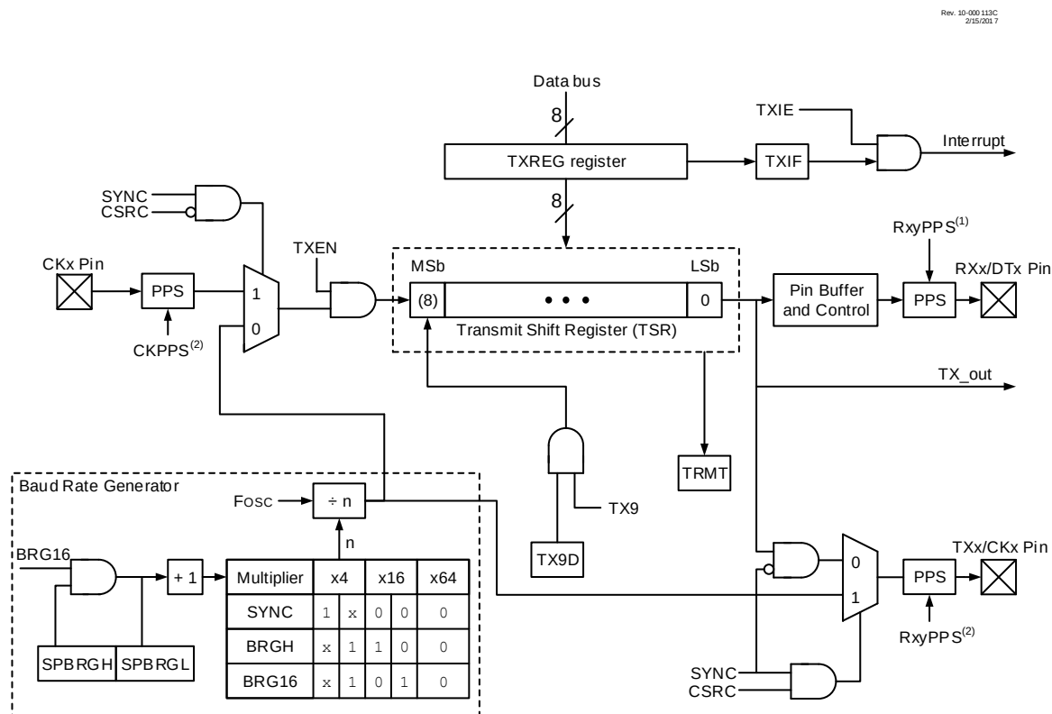
Figure 33-1. EUSART Transmit Block Diagram
