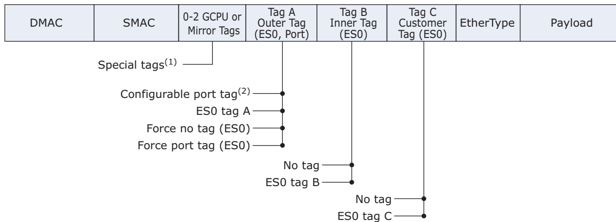
Figure 80 • VLAN Pushing
