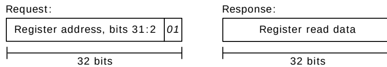
Figure 90 • WRITE Command
