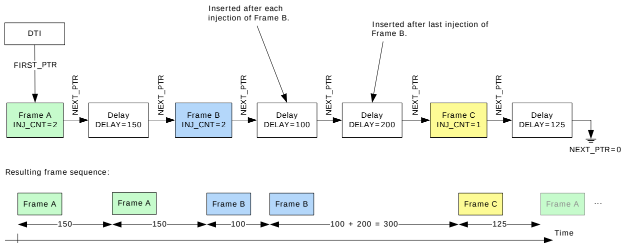
Figure 71 • DTI Frame/Delay Sequence Example
