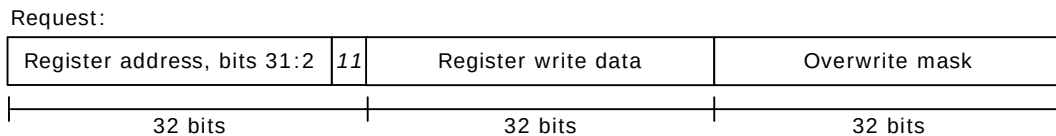
Figure 91 • READ-MODIFY-WRITE Command
