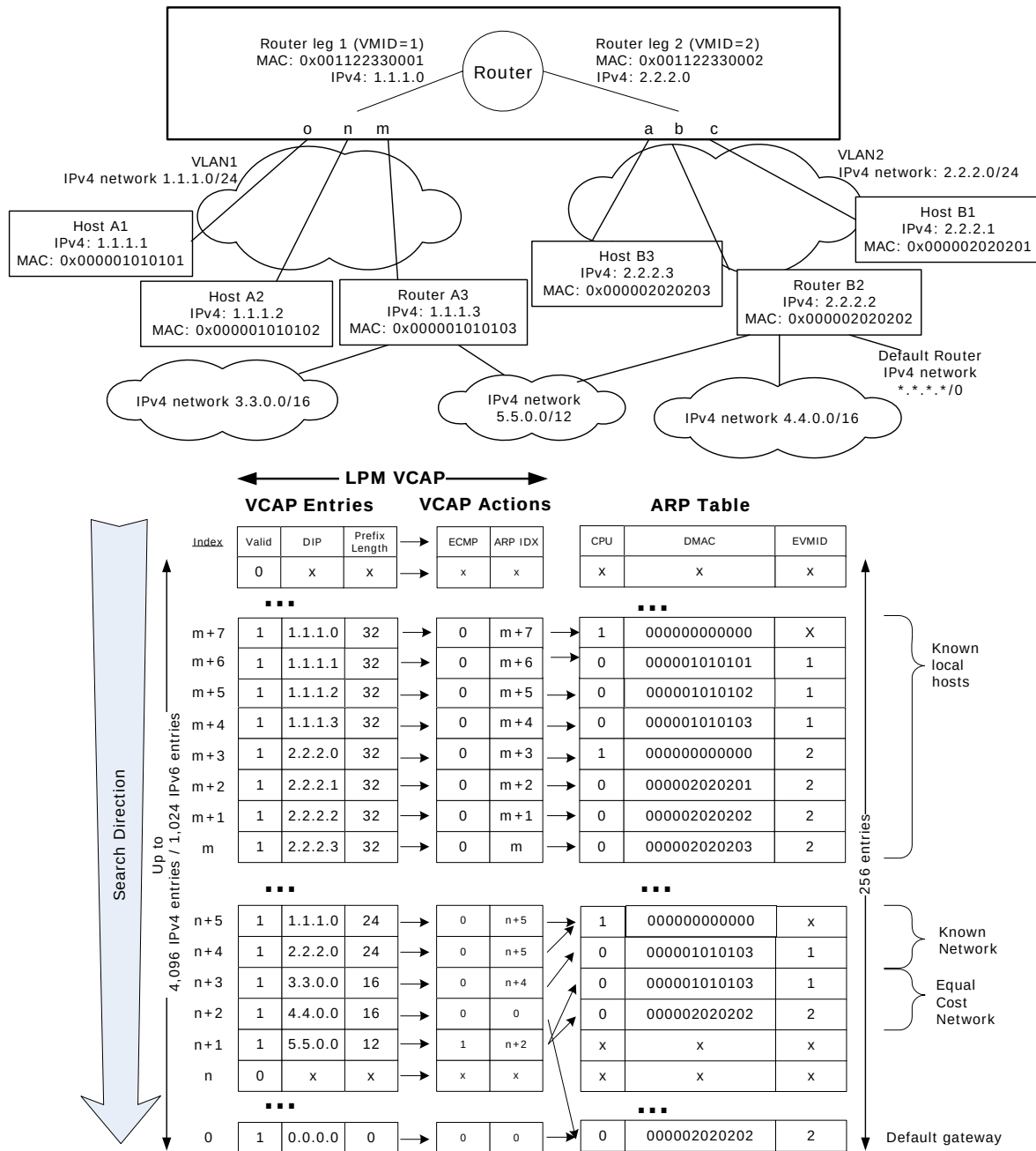
Figure 34 • IP Unicast Routing Example
