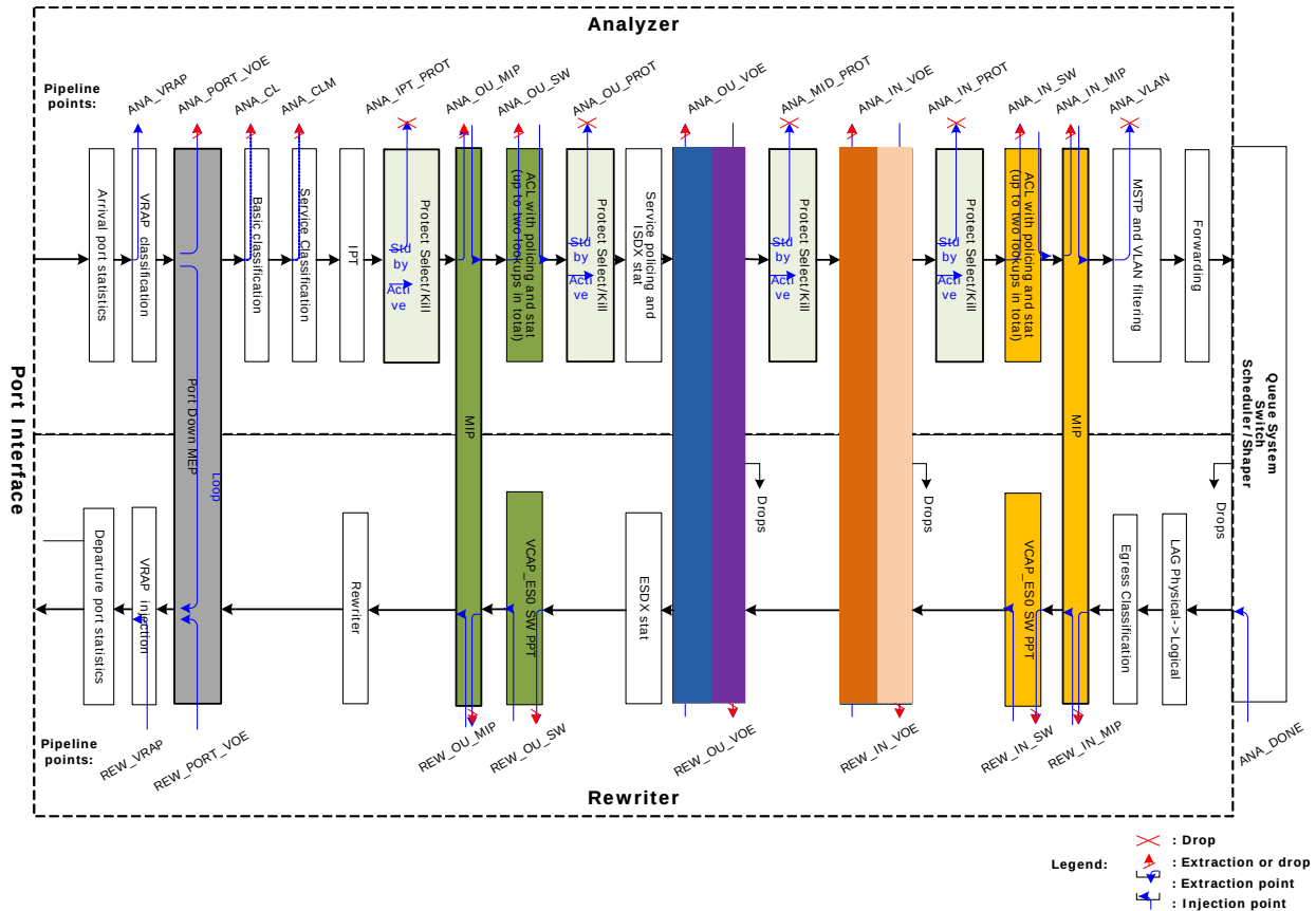
Figure 21 • Processing Flow
