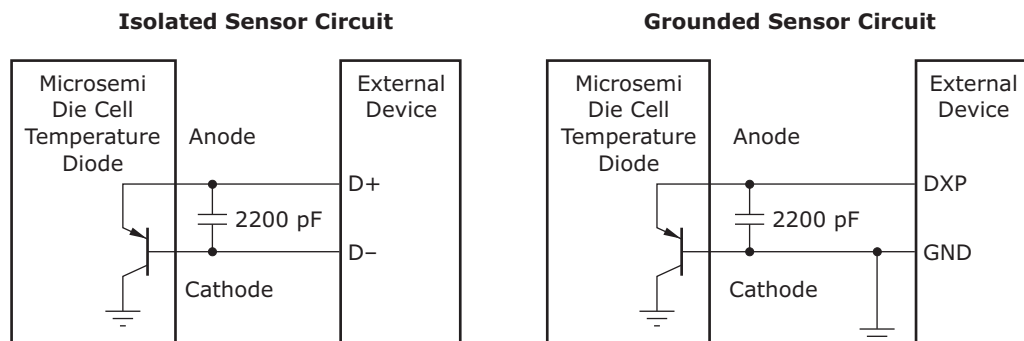
Figure 133 • Thermal Diode
