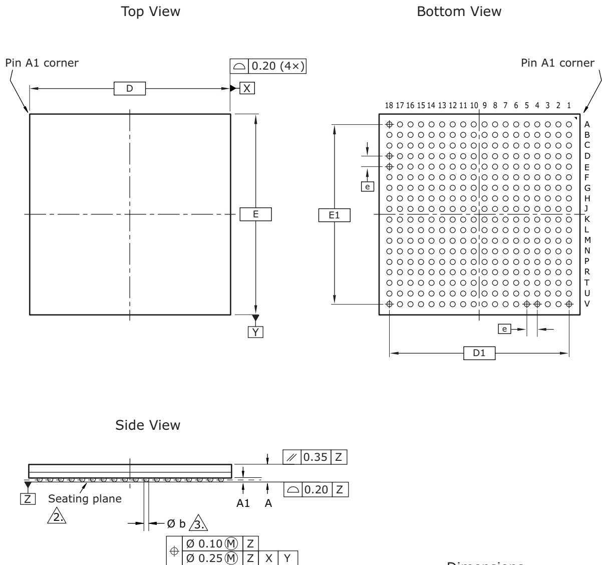
Figure 152 • Package Drawing
