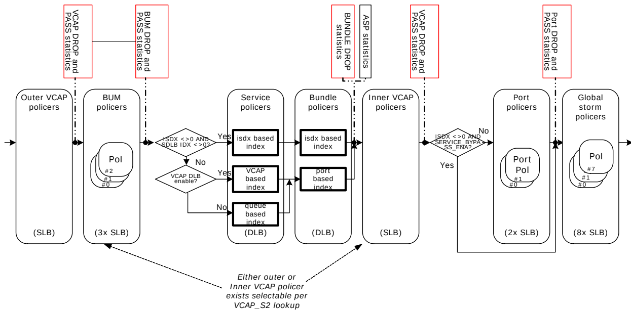
Figure 44 • Policer Hierarchy
