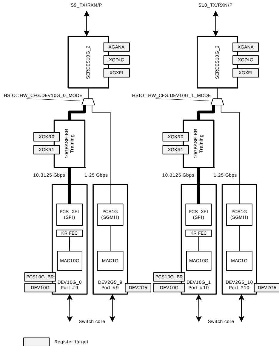
Figure 8 • 10G Muxing
