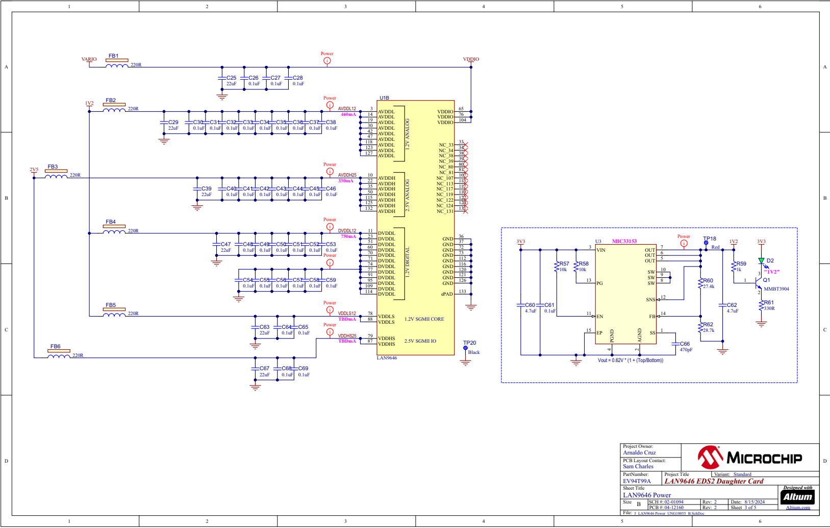
FIGURE A-3: LAN9646 EDS2 DAUGHTER CARD POWER
