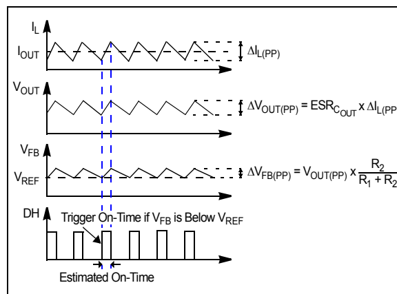
FIGURE 4-1: MIC28515 Control Loop Timing (CCM Mode).
