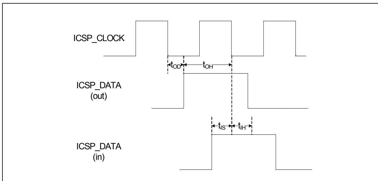
FIGURE 43-11: ICSP SETUP & HOLD PARAMETERS
