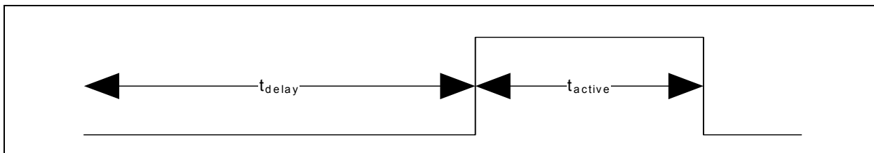
FIGURE 43-6: CPU_RESET TIMING
