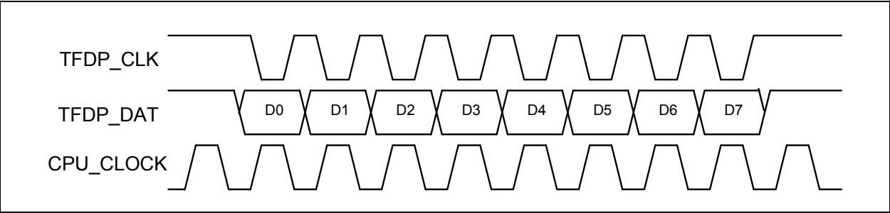
FIGURE 31-3: DATA TRANSFER
