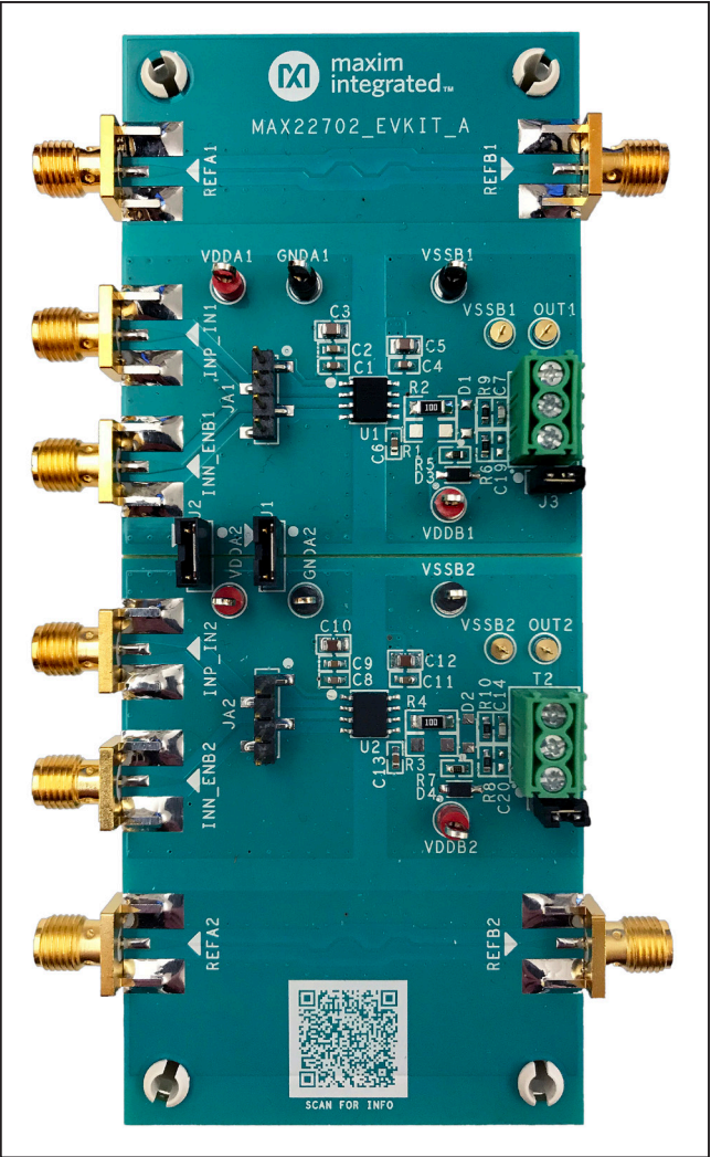
Figure 2. MAX22702EVALKIT#
