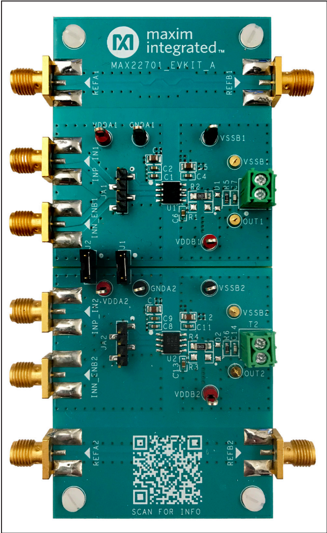
Figure 1. MAX22701EVALKIT#
