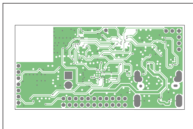
MAXSensorBLE_EVKIT—L03_SIGS
