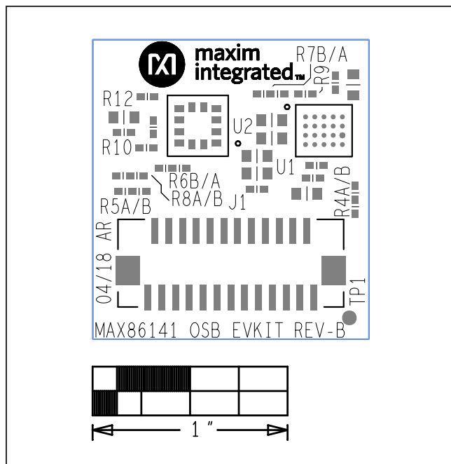
MAX86141OSBEK#—Silk_Top
