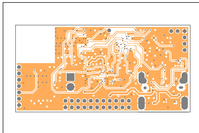
MAXSensorBLE_EVKIT—L05_SIGS
