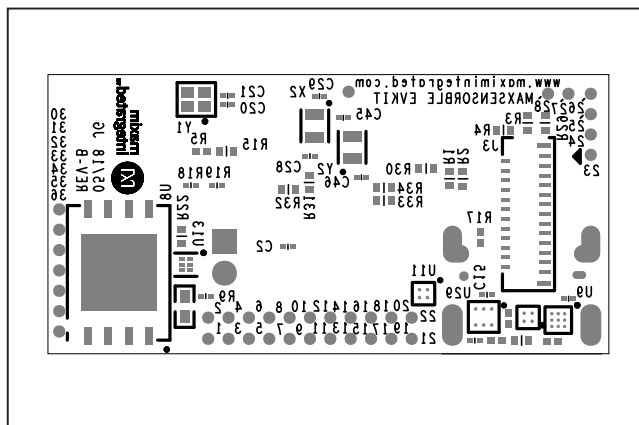
MAXSensorBLE_EVKIT—SILK_BOT
