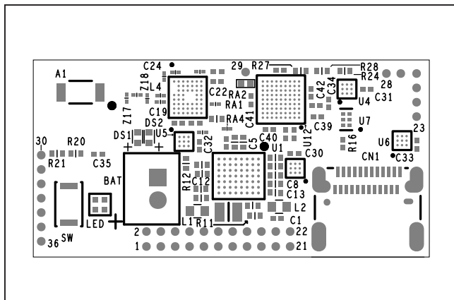
MAXSensorBLE_EVKIT—Silk_Top
