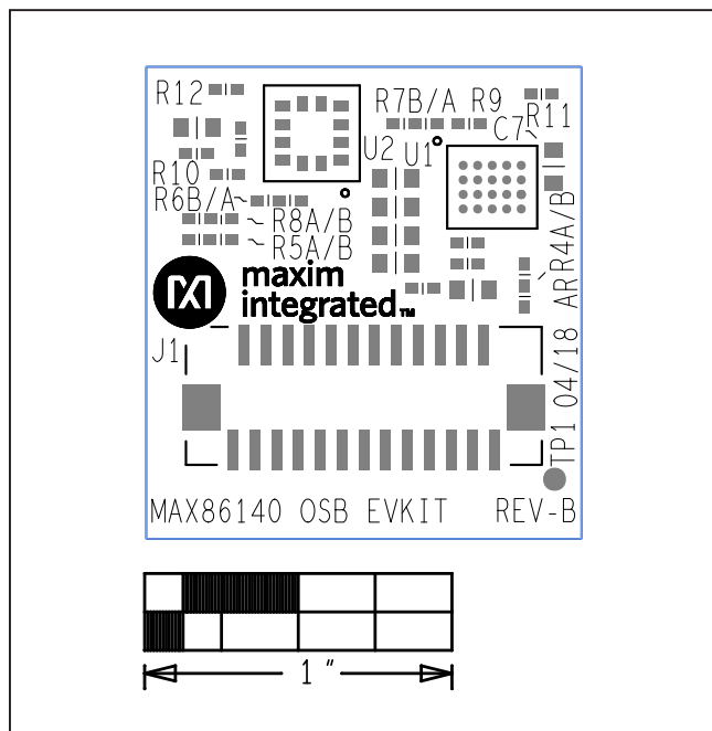
MAX86140OSBEK#—SILK_TOP
