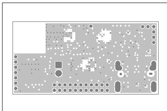
MAXSensorBLE_EVKIT—L02_GND
