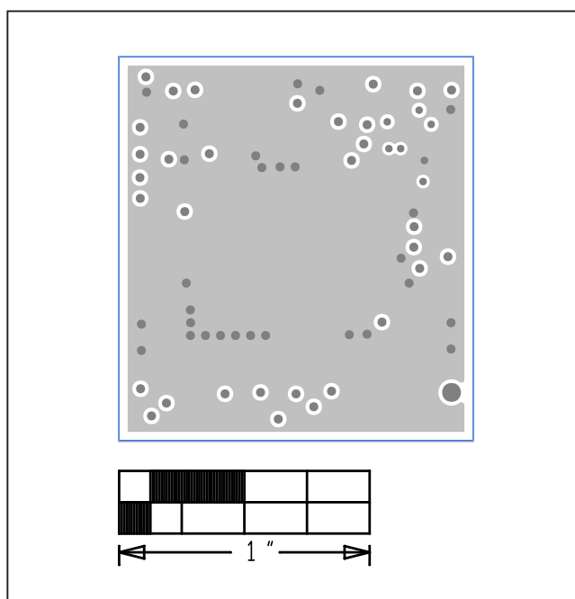
MAX86140OSBEK#—L02_GND
