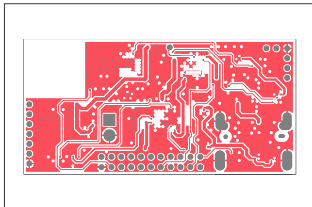
MAXSensorBLE_EVKIT—L04_SIGS
