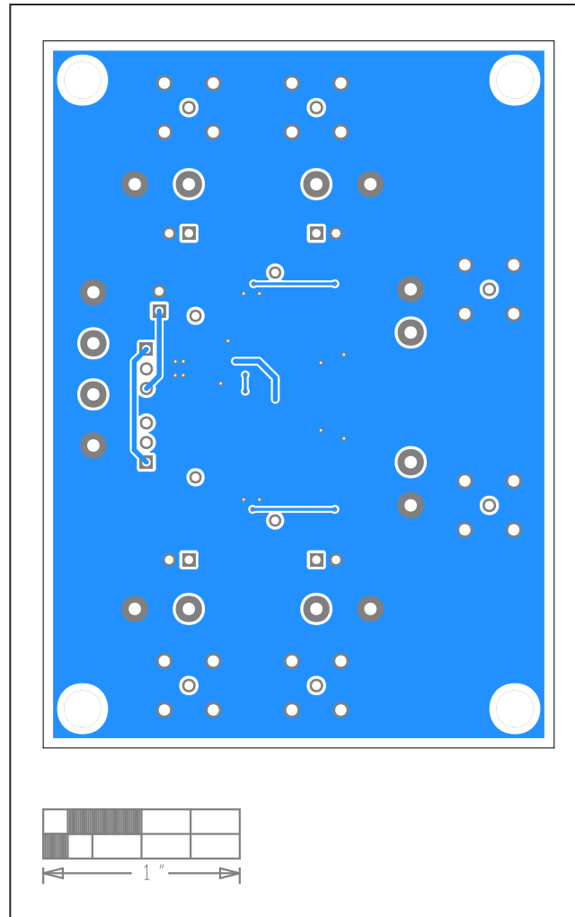
MAX40263 EV Kit PCB Layout—Bottom
