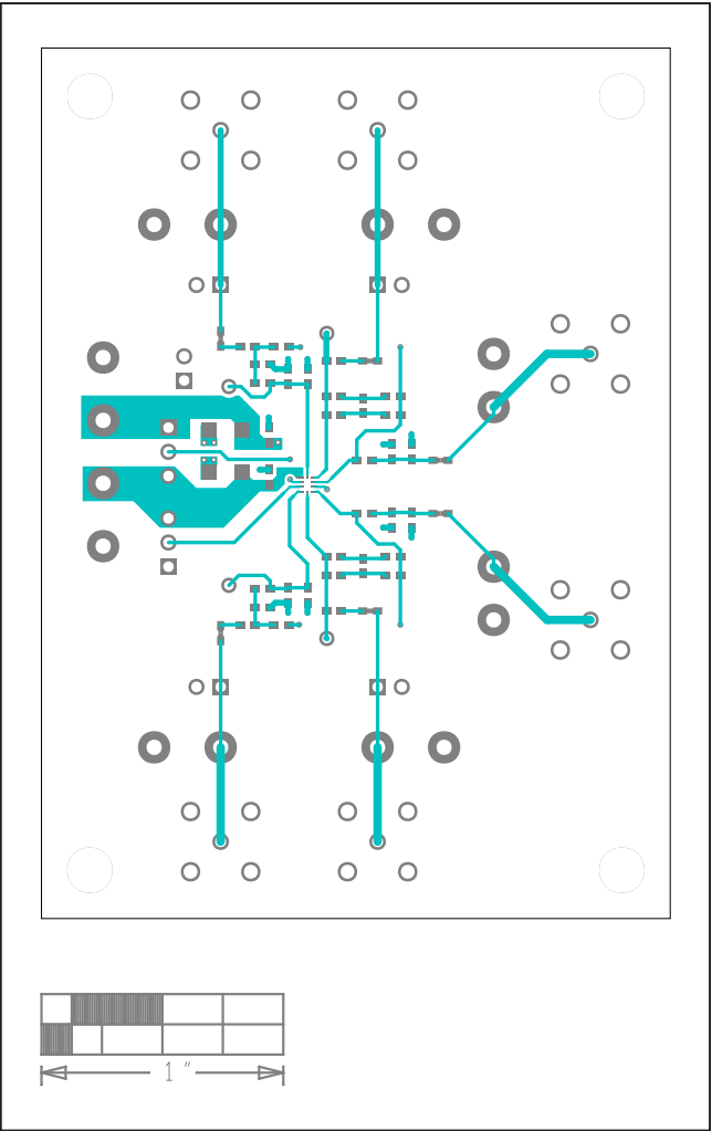
MAX40263 EV Kit PCB Layout—Top
