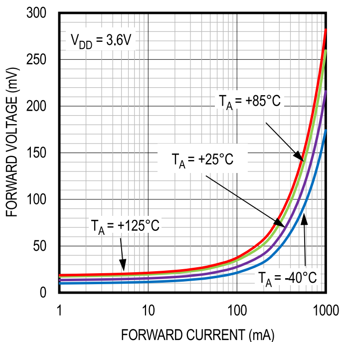
Figure 1. Forward Voltage vs. Forward Current
