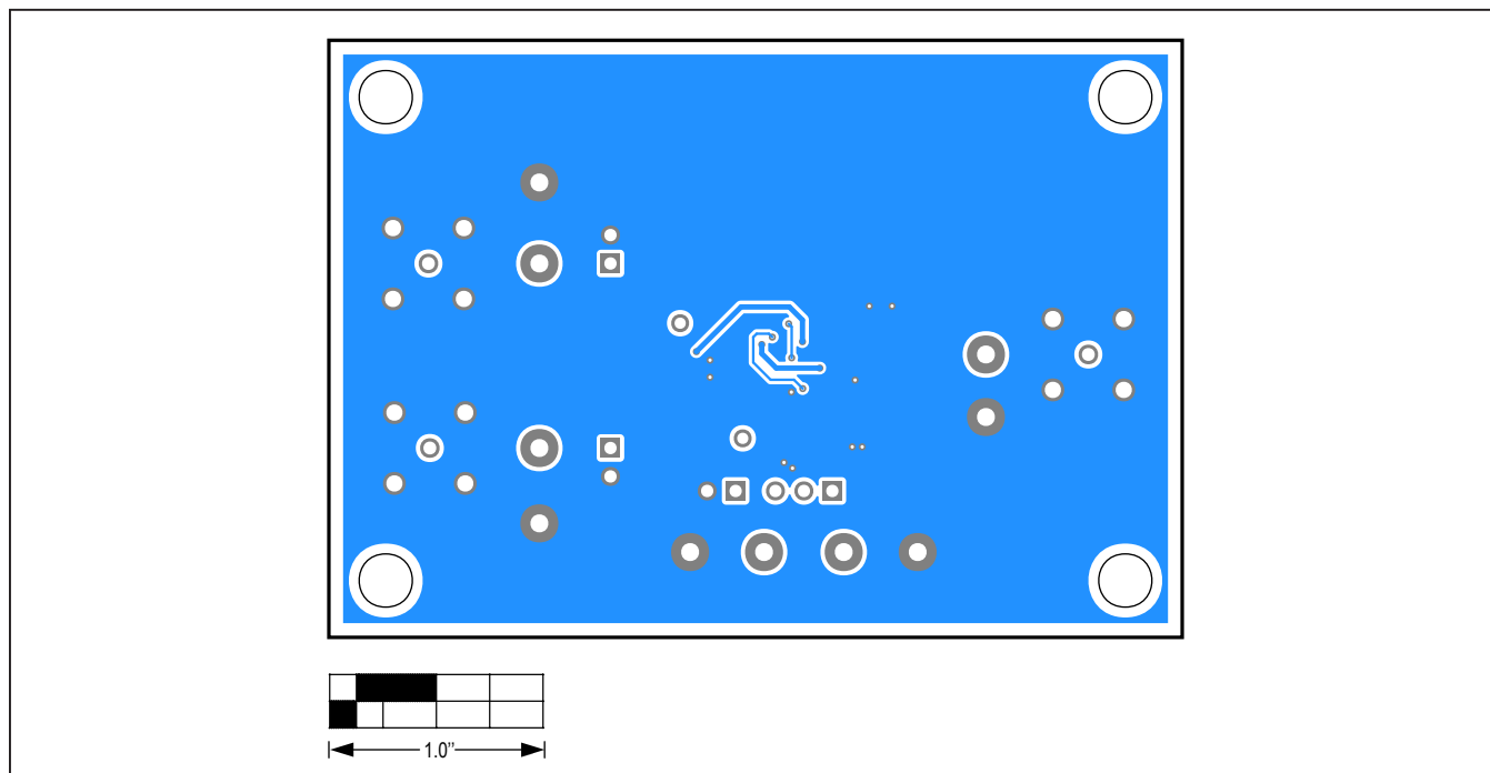
MAX40111 EV PCB Layout Diagram—Bottom View
