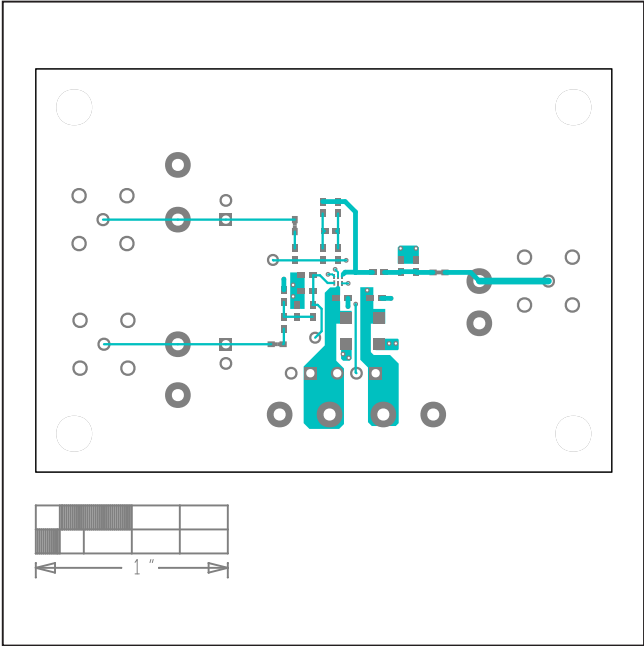
MAX40110 EV Kit PCB Layout—Top
