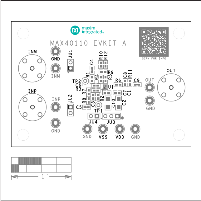
MAX40110 EV Kit PCB Layout—Silk Top
