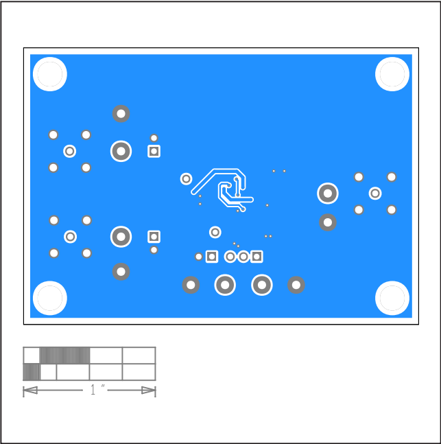
MAX40110 EV Kit PCB Layout—Bottom
