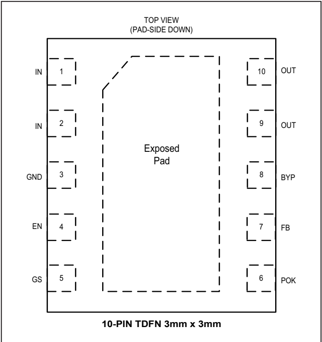
Figure 2. MAX38903B Pin Configuration
