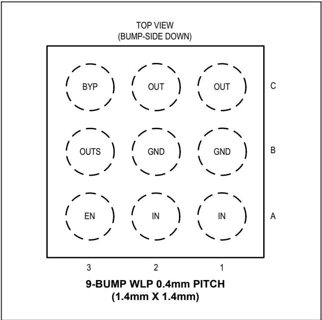
Figure 4. MAX38903D Pin Configuration
