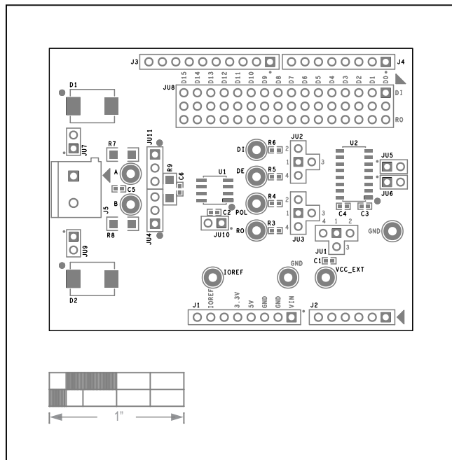
Silk Top
