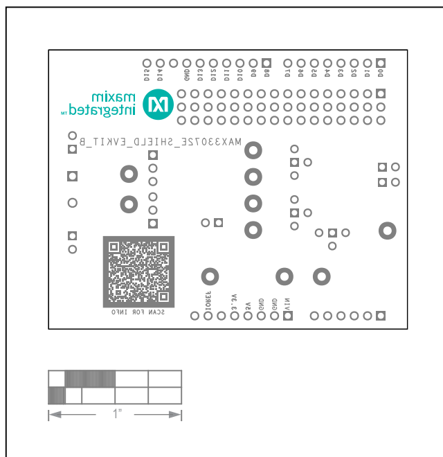
Silk Bottom
