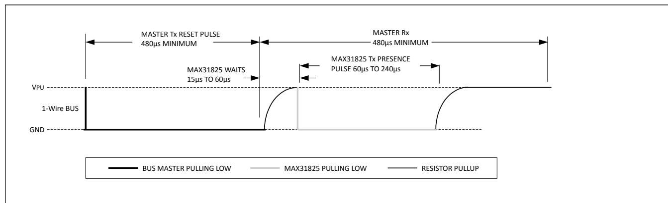
Figure 9. Initialization Timing
