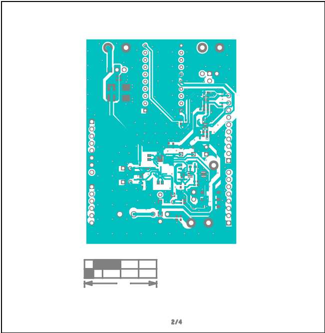
MAX31331 EV Kit PCB Layout—Top Layer
