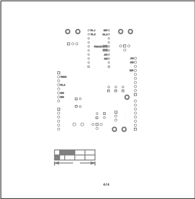
MAX31331 EV Kit PCB Layout—Bottom Silkscreen
