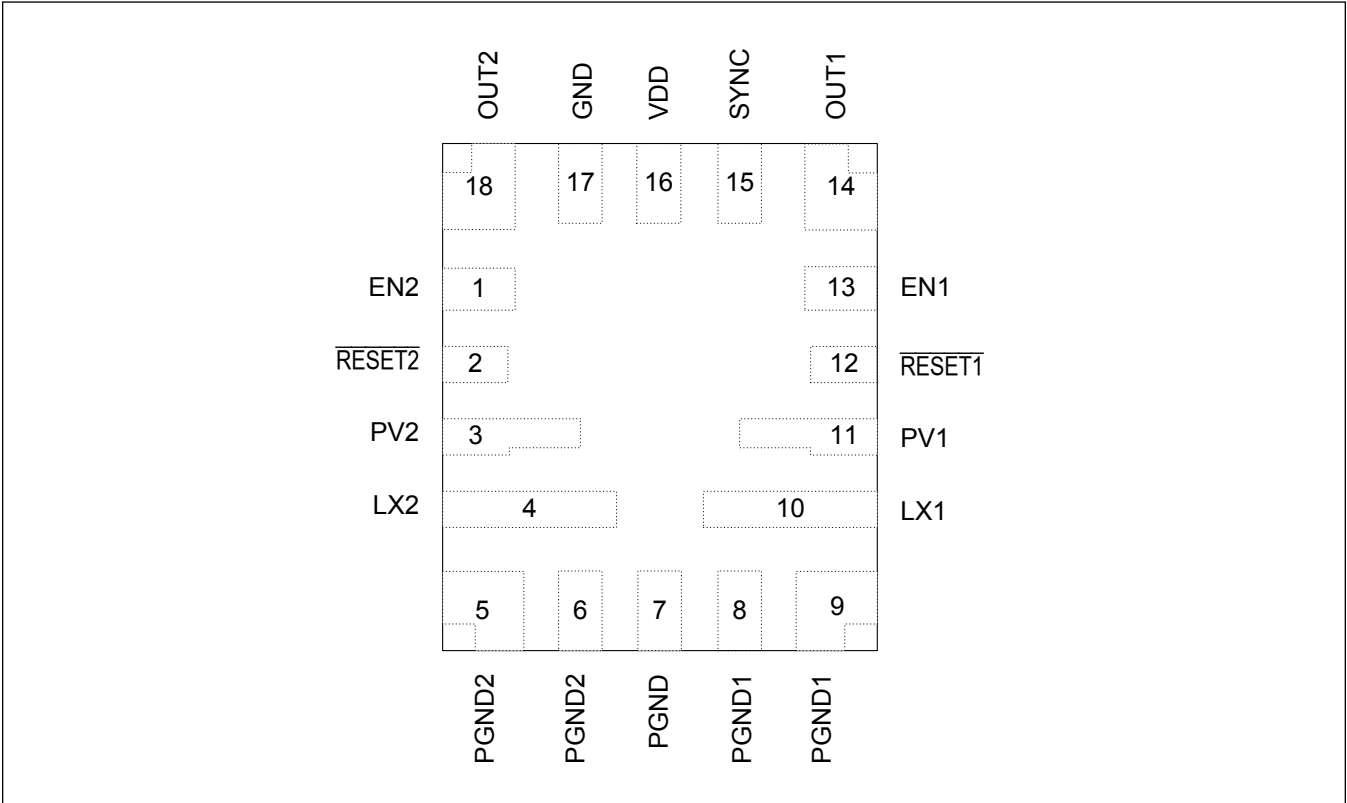
MAX20429 TOP VIEW
