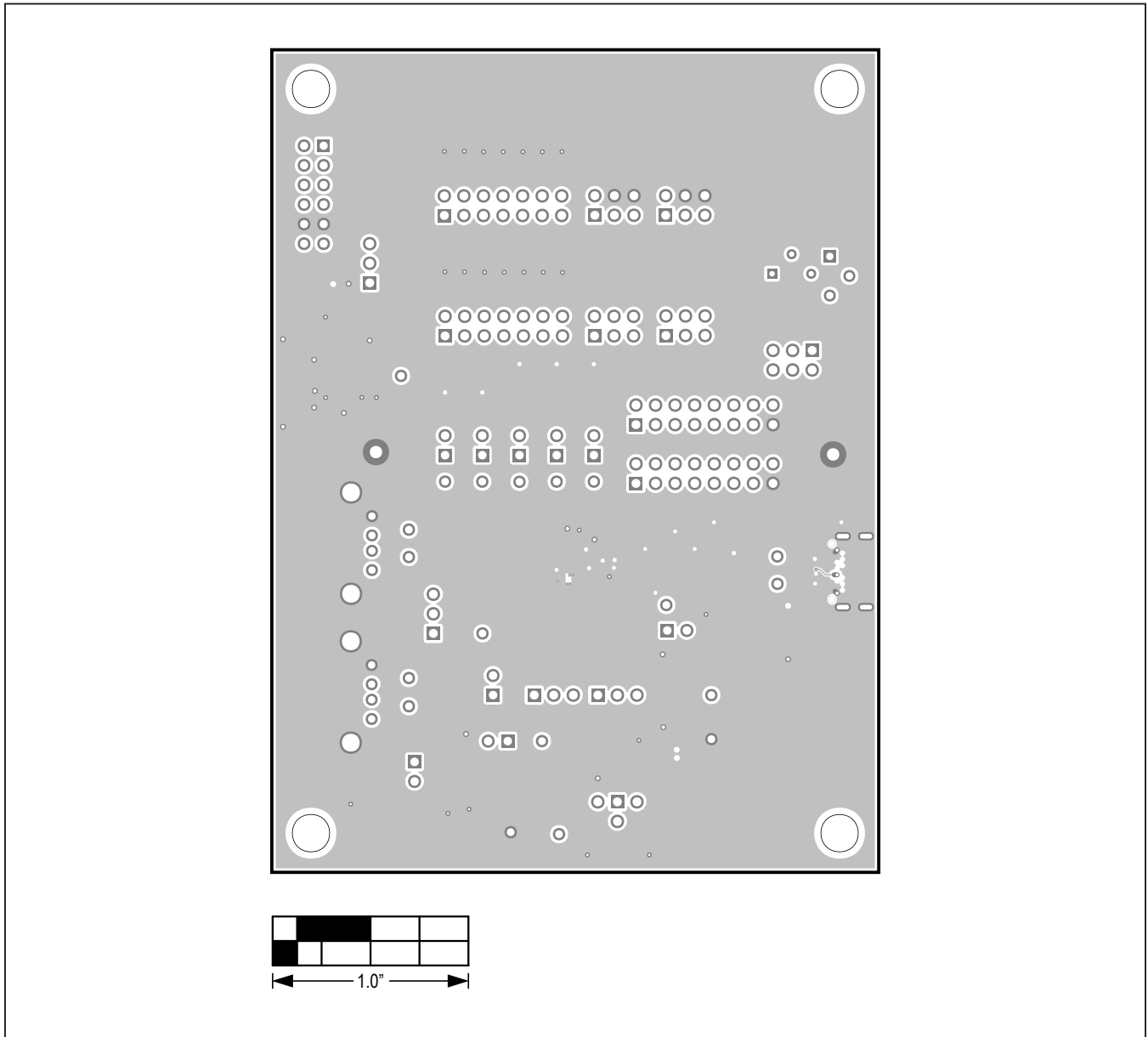
MAX20342 EV Kit PCB Layout—Layer GND
