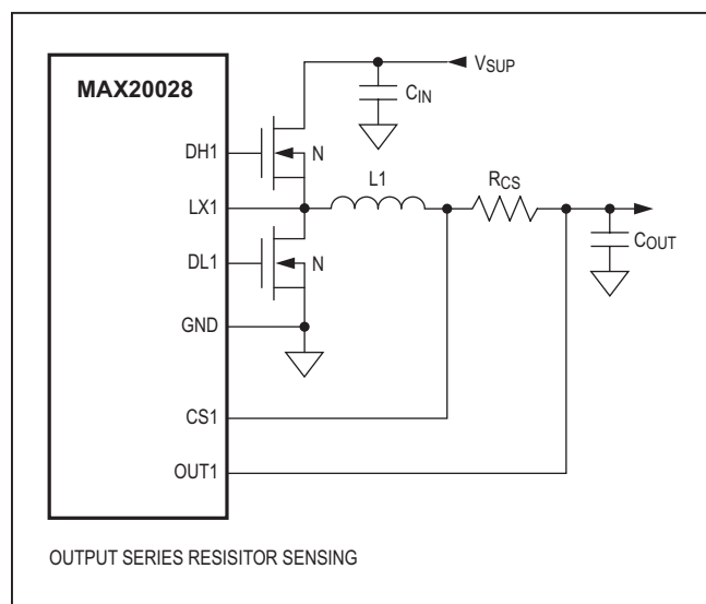
Figure 2. Current-Sense Configuration
