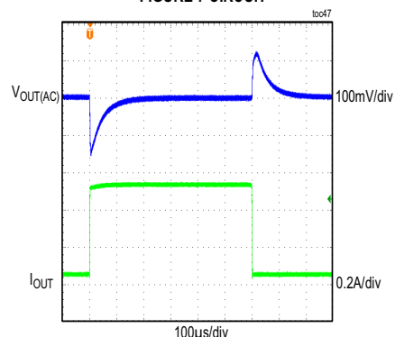
MAX17630C LOAD TRANSIENT BETWEEN 20mA AND 0.5A FIGURE 7 CIRCUIT
