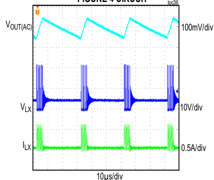
MAX17630C STEADY-STATE PERFORMANCE FIGURE 4 CIRCUIT
