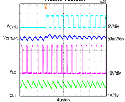
MAX17630B EXTERNAL CLOCK SYNCHRONIZATION FIGURE 4 CIRCUIT
