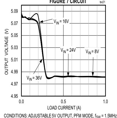
MAX17630C LOAD AND LINE REGULATION FIGURE 7 CIRCUIT t0c21
