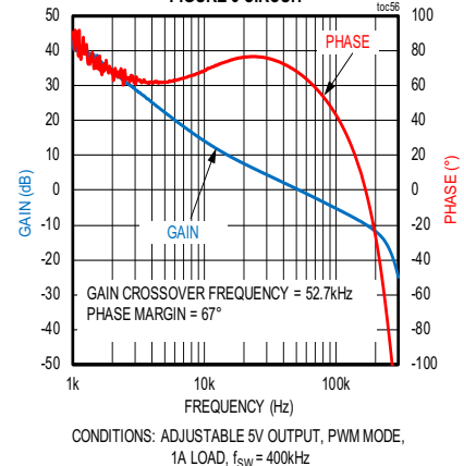
MAX17630C CLOSED-LOOP BODE PLOT FIGURE 6 CIRCUIT
