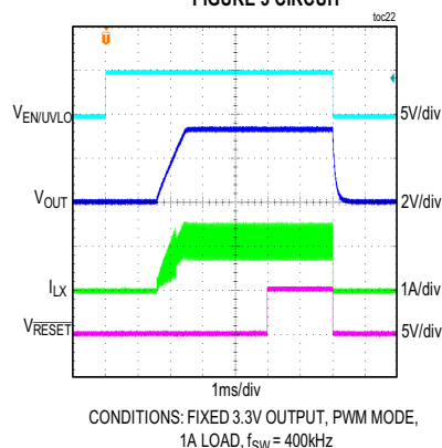
MAX17630A SOFT-START/SHUTDOWN FROM EN/UVLO FIGURE 3 CIRCUIT t0c22
