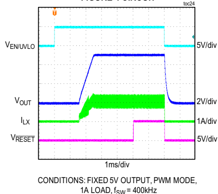
MAX17630B SOFT-START/SHUTDOWN FROM EN/UVLO FIGURE 4 CIRCUIT t0c24
