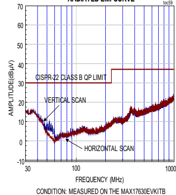
MAX17630B, 5V OUTPUT, 1A LOAD CURRENT RADIATED EMI CURVE
