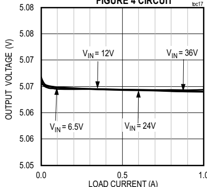
MAX17630B LOAD AND LINE REGULATION FIGURE 4 CIRCUIT
