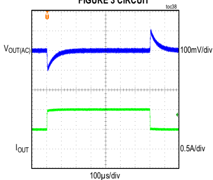
MAX17630A LOAD TRANSIENT BETWEEN 0.5A AND 1A FIGURE 3 CIRCUIT
