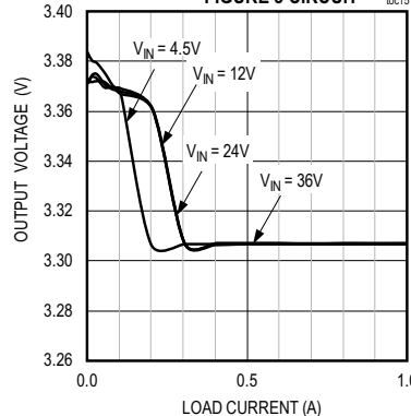
MAX17630A LOAD AND LINE REGULATION FIGURE 3 CIRCUIT
