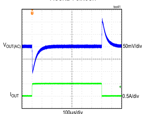
MAX17630B LOAD TRANSIENT BETWEEN 0A AND 0.5A FIGURE 4 CIRCUIT
