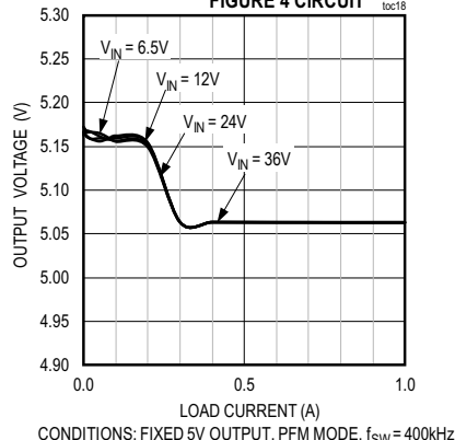
MAX17630B LOAD AND LINE REGULATION FIGURE 4 CIRCUIT t0c18
