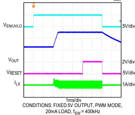
MAX17630B SOFT-START WITH PREBIAS VOLTAGE OF 2.5V FIGURE 4 CIRCUIT t0c25
