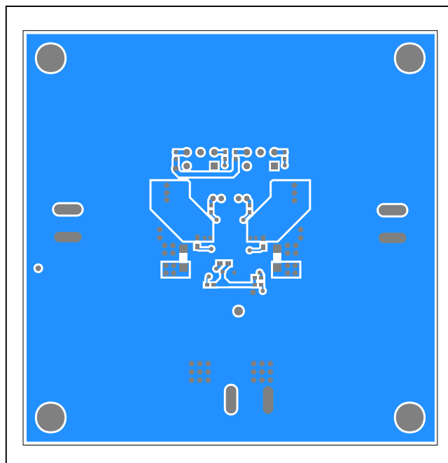
MAX17509 EV Kit—Bottom
