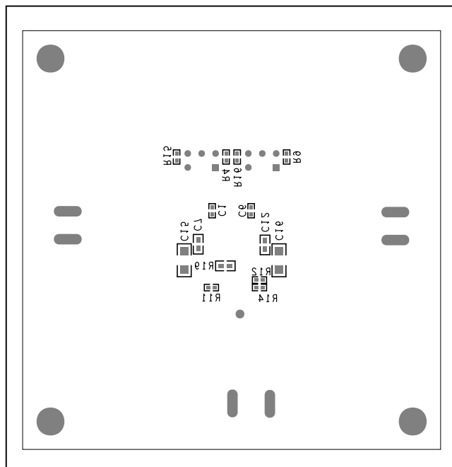
MAX17509 EV Kit—Bottom Silkscreen
