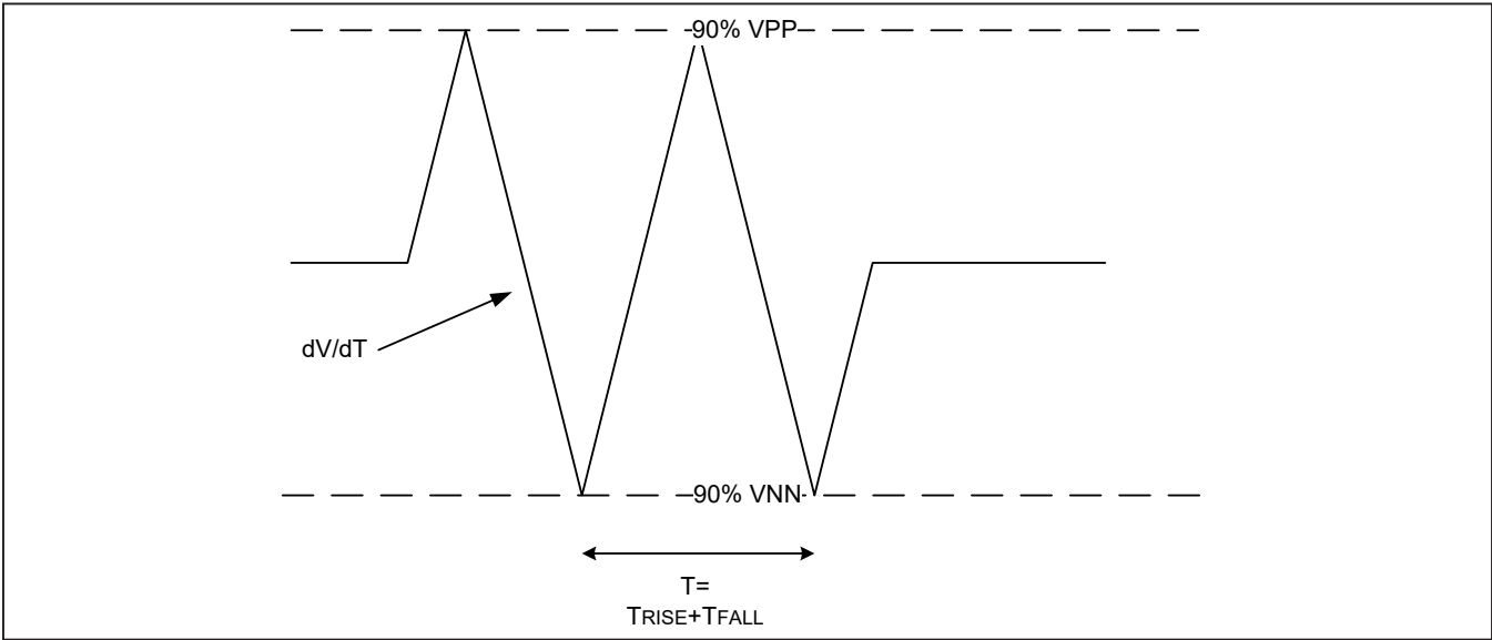
Figure 3. Bandwidth Diagram
