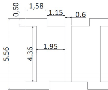
Soldering patterns
