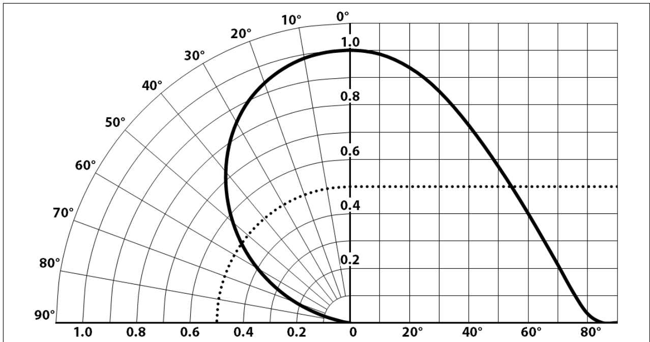
Radiation Pattern 9
