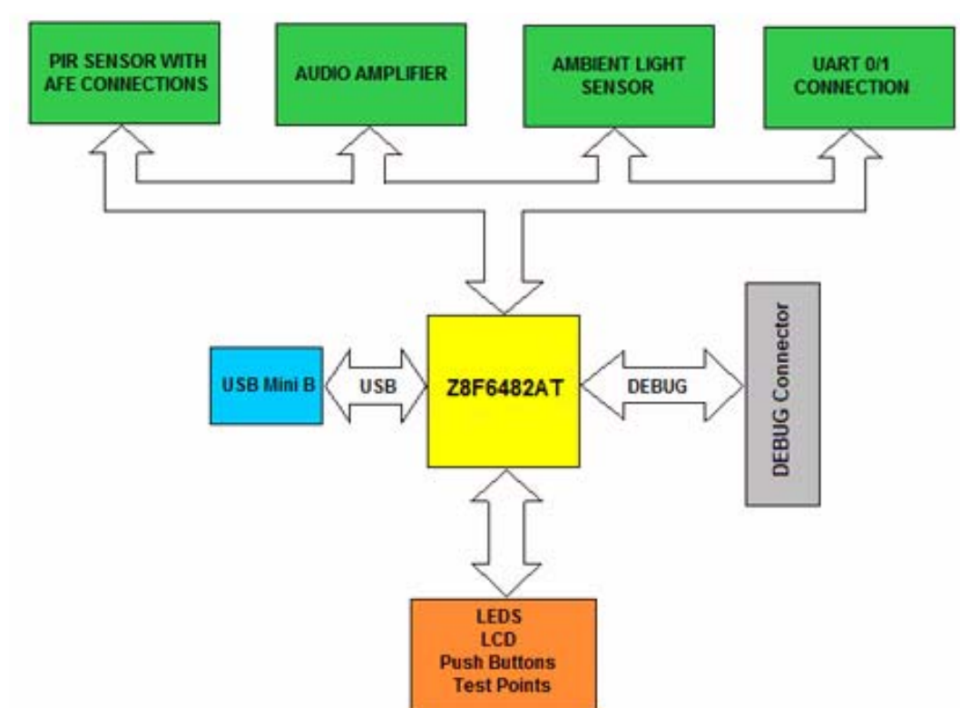
Figure 13. F6482 Series Development Kit Block Diagram
