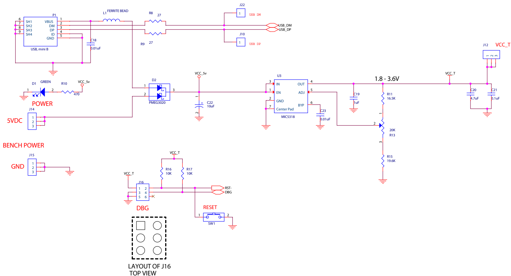
Figure 37. F6482 Series Development Board Schematic Diagram, #1 of 4
