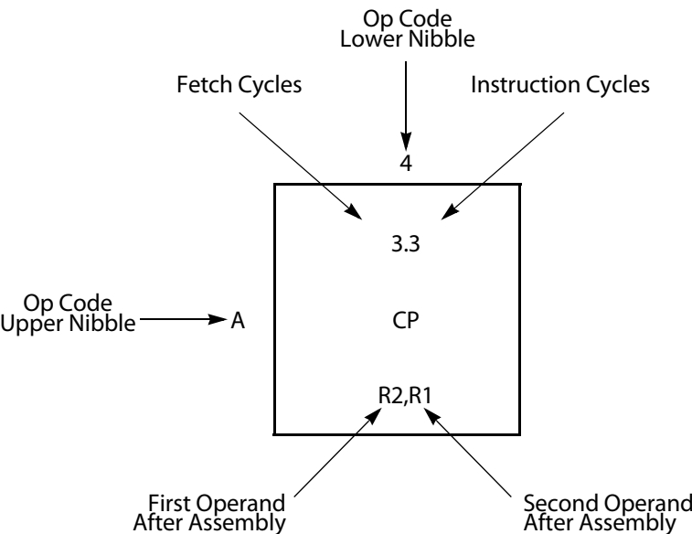
Figure 68. Op Code Map Cell Description
