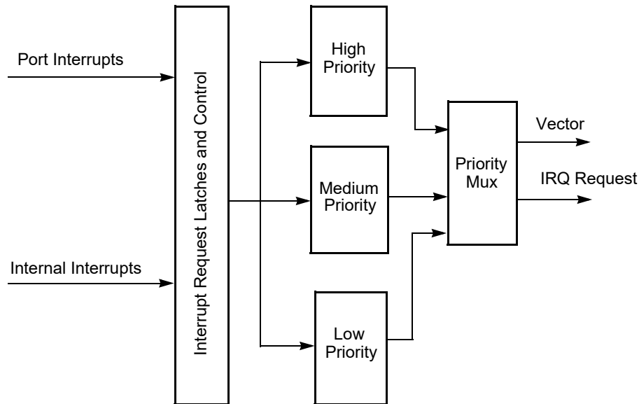
Figure 12. Interrupt Controller Block Diagram
