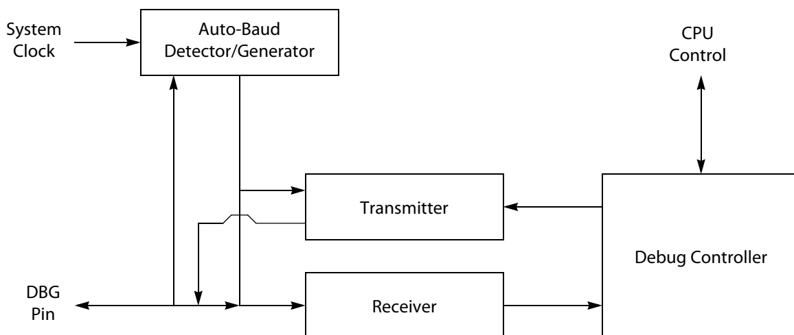
Figure 64. On-Chip Debugger Block Diagram
