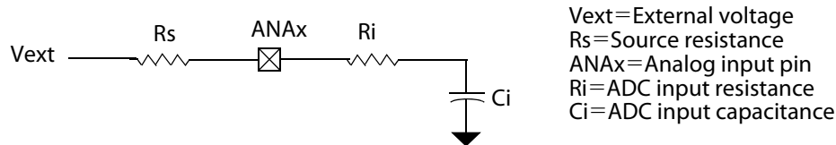
Figure 56. ADC Input Equivalent Circuit
