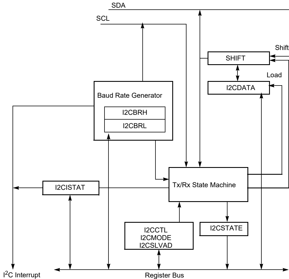
Figure 41. I²C Controller Block Diagram
