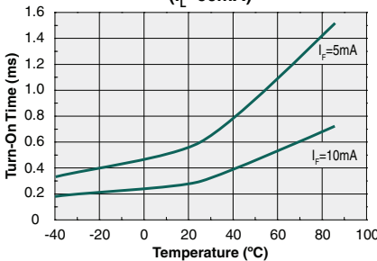
Typical Turn-On Time vs. Temperature ( I_L=60mA )
