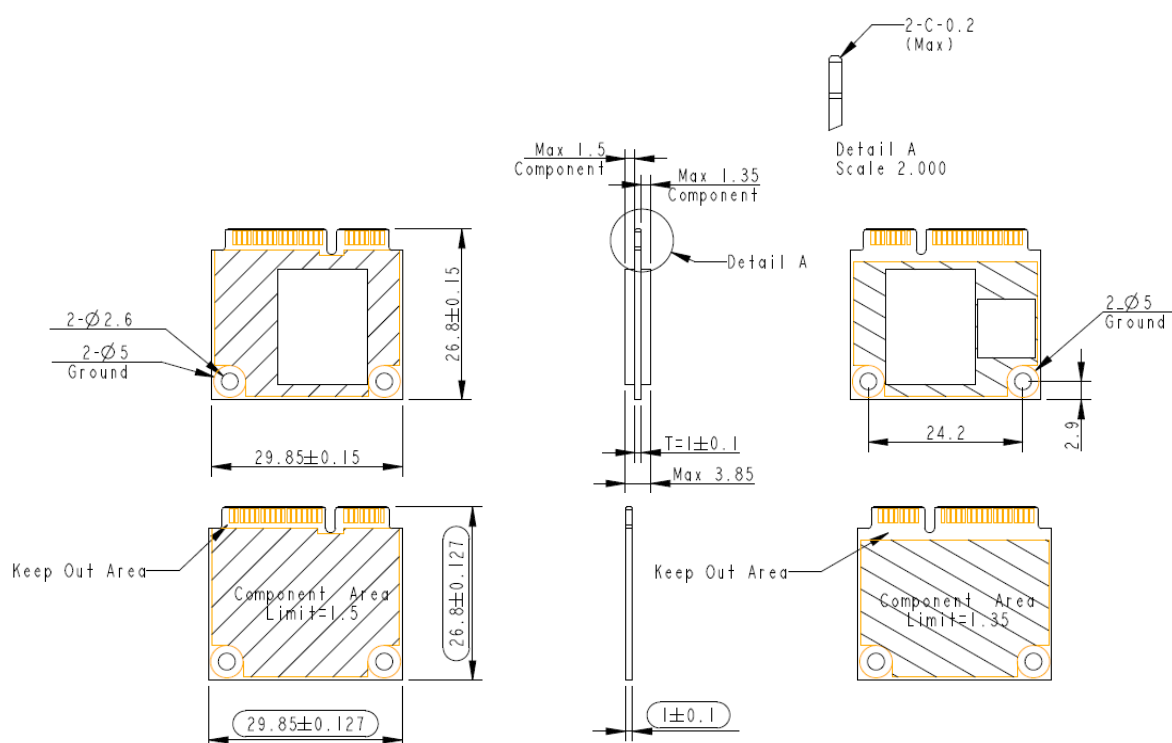
Figure 9-1 Physical Dimensions
